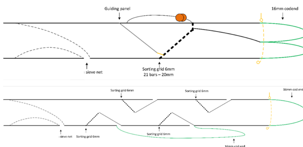
Figure 12.9.1 The single grid design after the design tested for the Nephrops fishery (above) and the design with four smaller grids (below).
