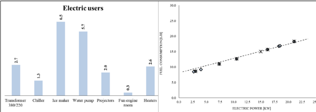
Figure 126.15.2. Power demand of electric users.
