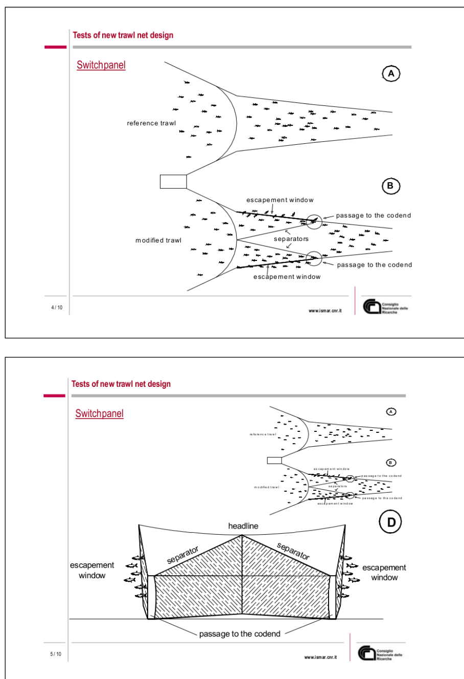
Figure 10.19: summary of presentation, given by Antonello Sala: Tests of a new trawl net design (which guides the fish to the side panels) – preliminary results of sea trials in the Mediterranean Sea.
