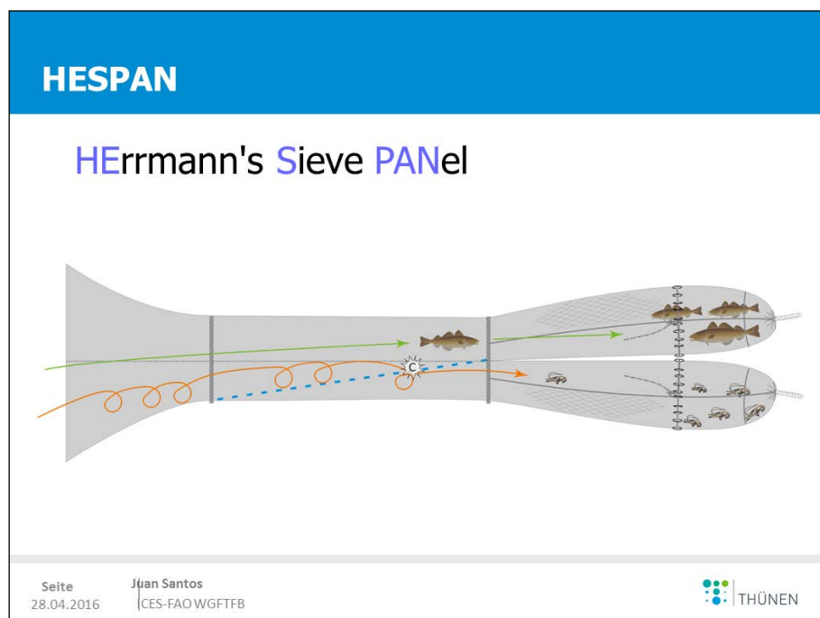
Figure 10.10: summary of presentation, given by Juan Santos (slide 1): Schematic drawing of a selection device to separate Nephrops from fish (HESPAN).
