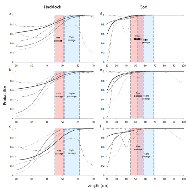
Figure 10.16: summary of presentation, given by Bent Herrmann (SINTEF; Denmark): Stimulation-induced selectivity.
