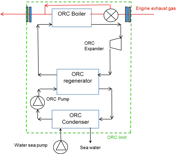
Figure 242.15.1. ORC system architecture.
