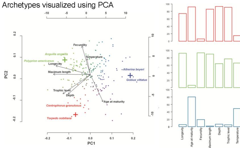
Figure 6.10. Biplot of the PCA performed on the seven traits. The archetypes are visualized as colored crosses. Each species is represented by a point, in which color is a proportional combination of the colors of the archetypes (left). Barplots visualizing the percentage of the traits used, to the archetypes (right).
