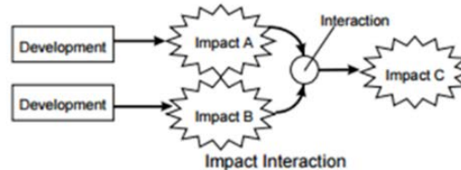
Figure 3. Flow diagrams illustrating indirect and cumulative impacts and impact interactions (Walker 1999).
