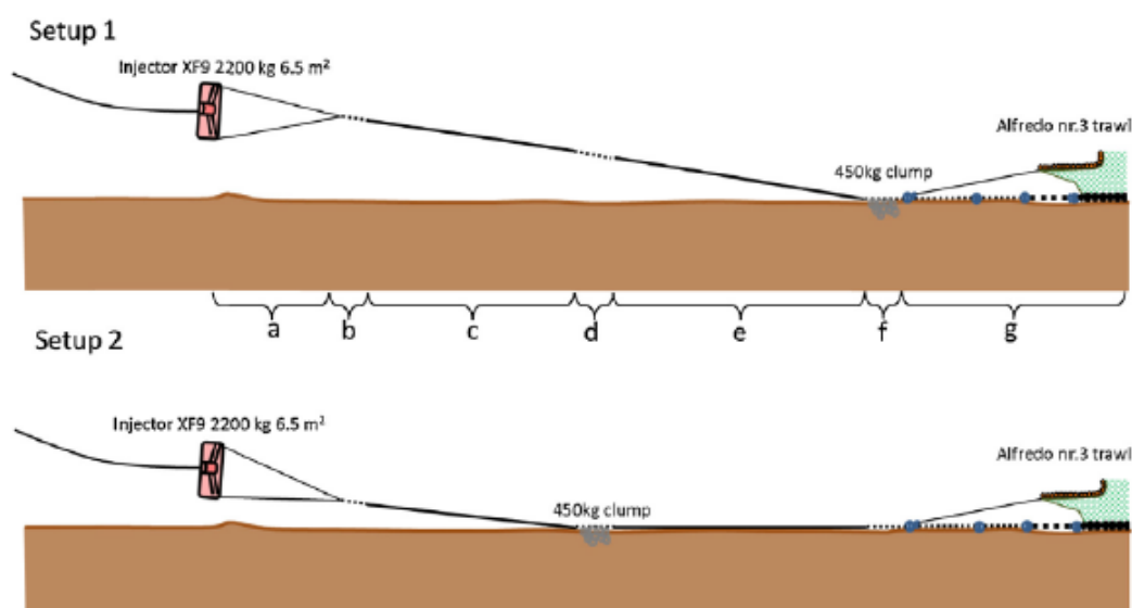
Schematic view of the gear used during the sea trials. (a) 15.9 m backstop, (b) 3 m backstop extension, (c) 30 m of 30 mm sweep, (d) 4 m of 19 mm chain (attaching position for the clumps), (e) 45 m of 30 mm sweeps, (f) 4 m of 19 mm chain (attaching position for the clumps), (g) 45 m of ground gear composed of 19 mm chain (32 mm chain closest to the rockhopper), and the rockhopper.
