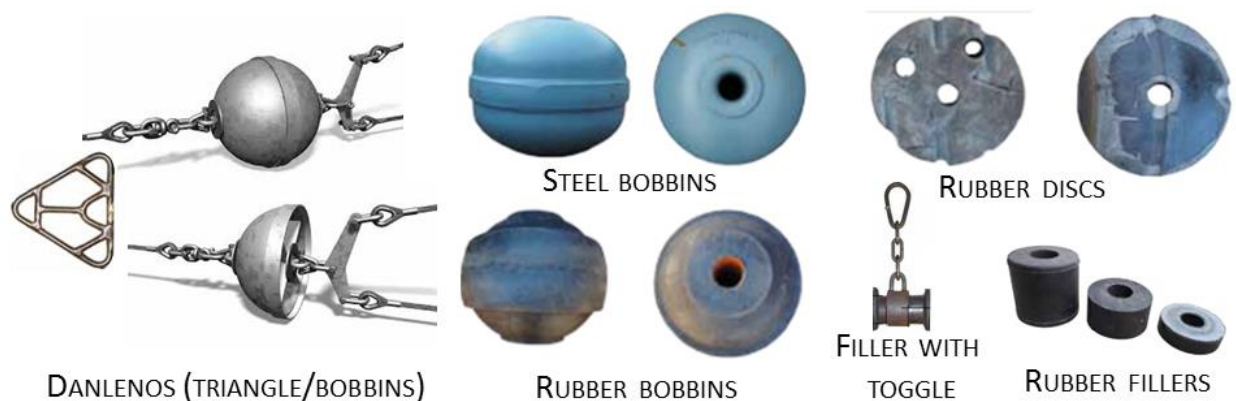
Fig 3.6: Examples of commonly used components on footropes/groundropes/gears for bottom trawling (images are copied from Galbraith and Rice 2004 8 and leaflets from various manufactures).
