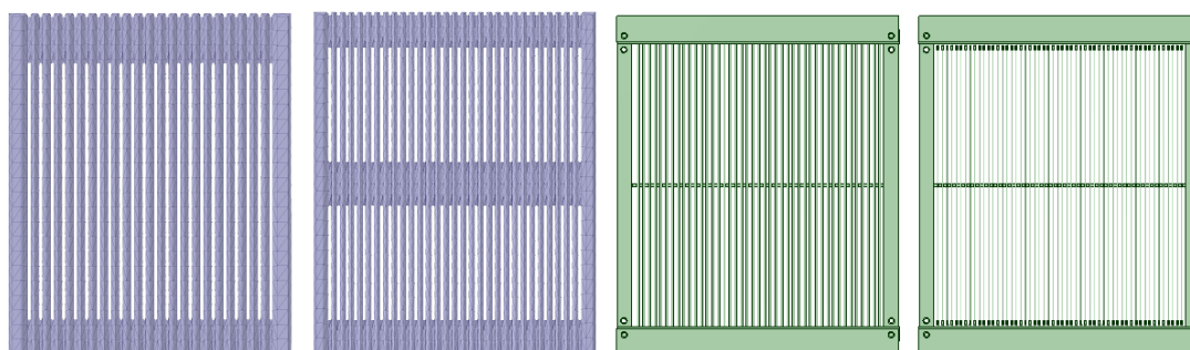
Figure 8.6.2: Grid-designs tested (Front view). From left to right: Plastic-grid 1(Dutch design, Type 1); Plastic-grid 2(Dutch design, Type 2); Fiberglass-dropshaped-grid; Steel-grid (2mm bar width)
