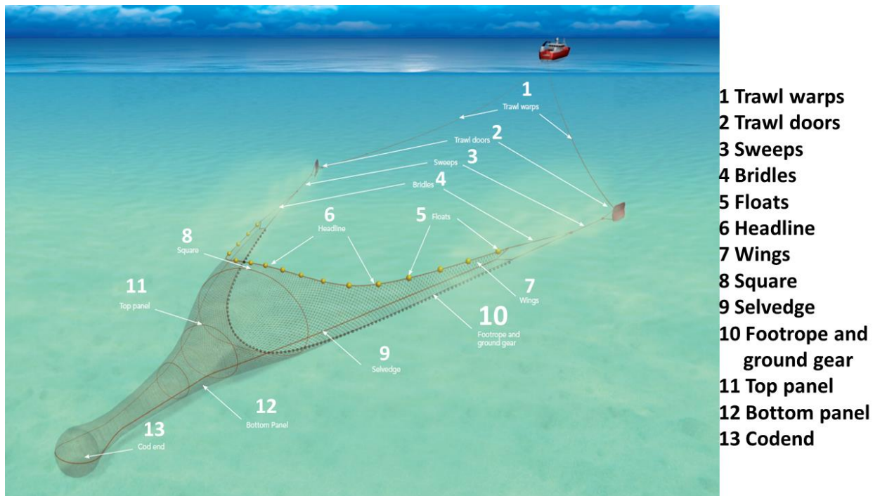
Fig 2.6: The basic components of an otter board bottom trawl system (Seafish Assetbank).
