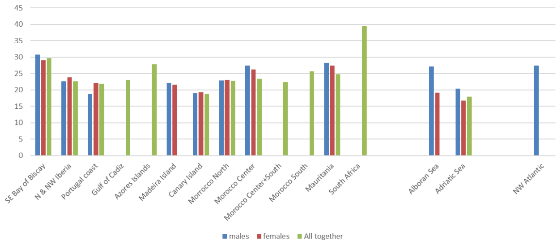
Figure 5.5.1. Average length at first maturity ( L_{50} ) estimated for chub mackerel, for males, females, or both sexes combined, for each area of distribution. Only studies presenting L_{50} values based on fish total length (TL) were considered in this plot (Table 5.5).
