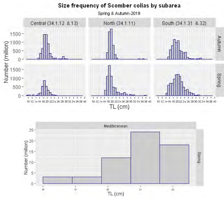
Figure 3.3.1.2. Size–frequency distribution of Scomber colias in the NW African coast (Morocco) (upper panel) and in the Moroccan Mediterranean area (lower panel) – Spring and Autumn 2019 surveys.
