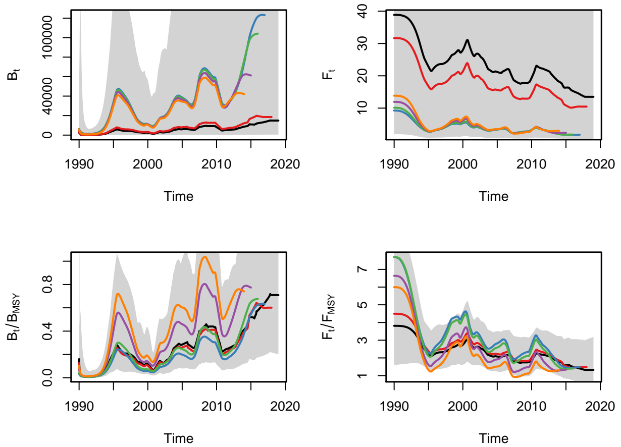
Figure 5: Retrospective analysis for scenario 1
