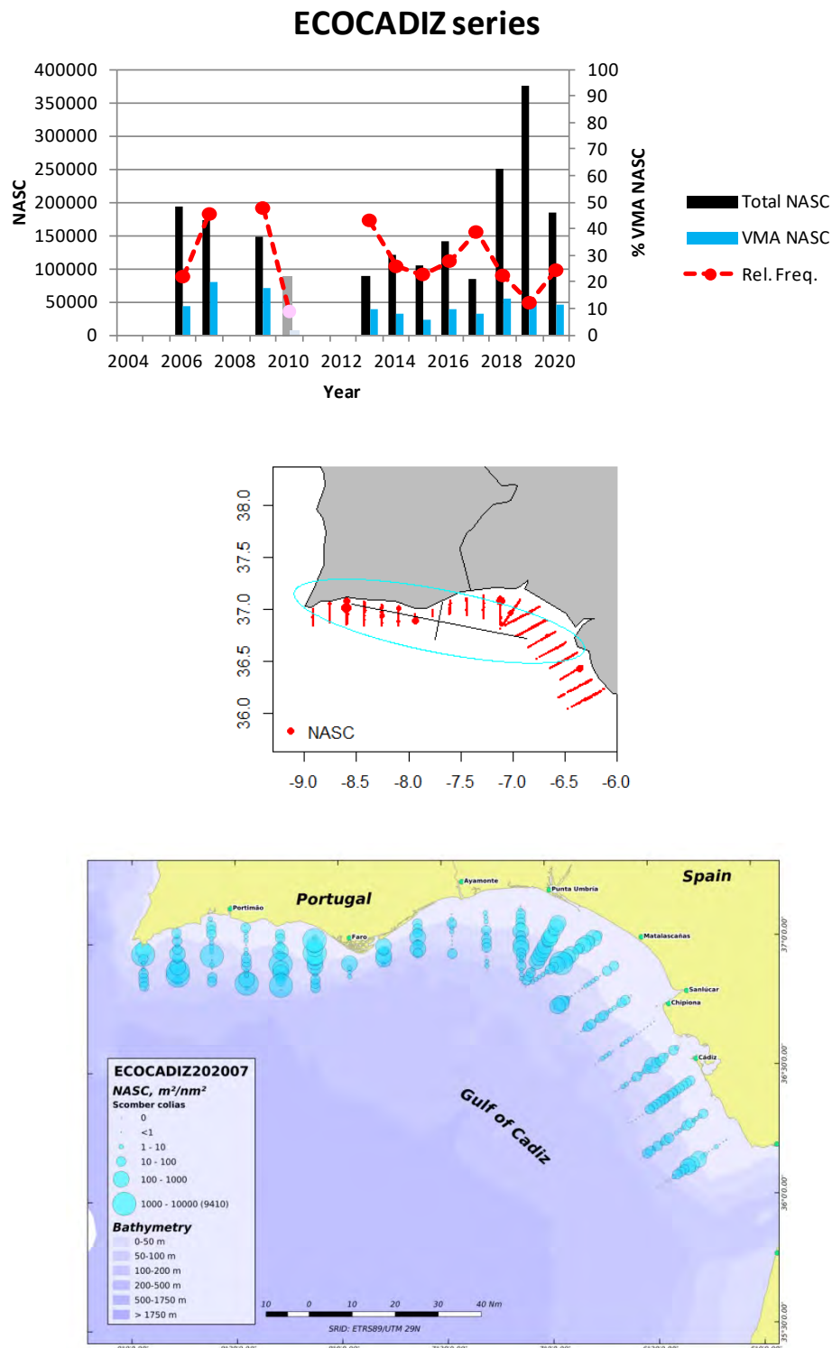
Figure 3.2.11. ECOCADIZ Summer acoustic-trawl survey series. ICES subdivisions 27.9.a.s.a and 27.9.a.s.c (Gulf of Cadiz). Upper panel: time-series of estimates of acoustic density (NASC estimates; m^2nm^{-2} ) differentiated between total NASC and NASC allocated to chub mackerel (VMA: FAO Alpha3 code for Scomber colias ). The 2010 survey only covered the Spanish and the Portuguese easternmost waters. Middle panel: location of the centre of gravity and the inertia of the species' distribution (pooled NASC data for years 2007–2015; sources: Canseco, 2016; Ramos and Carrera presentation during the WK; abstract without figures available in Annex 4). Bottom panel: acoustic densities (NASC, m^2nm^{-2} ) for chub mackerel in 2020.
