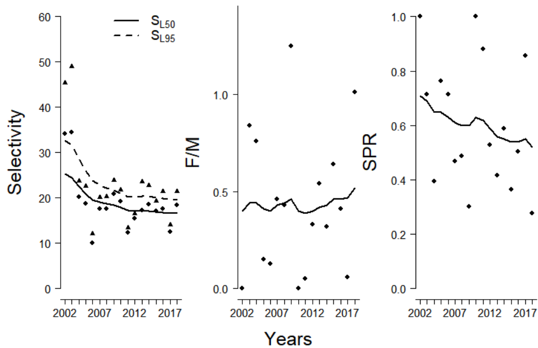
Figure 7.3.2.6.4. Moroccan central and southern chub mackerel stock: Estimated values for SPR, SL50, SL95 and F/M for scenario 2; the black line corresponds to the smoother line to the estimated points.
