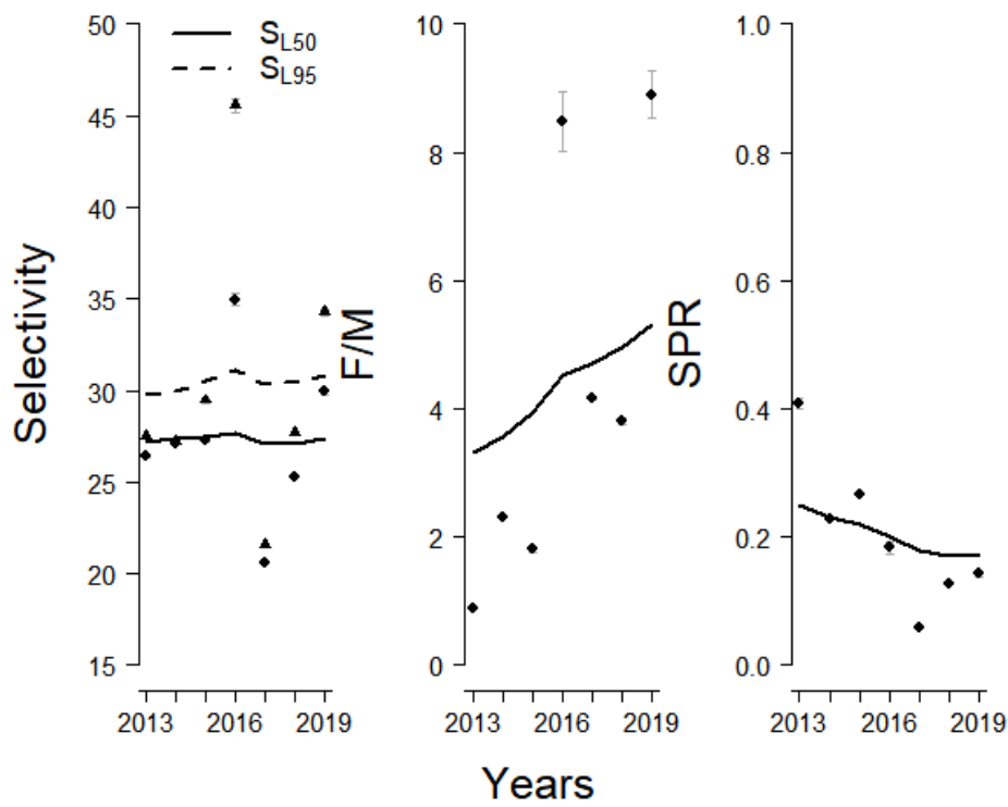
Figure 7.3.2.1.4. Cantabrian Sea (27.8.c) chub mackerel: Estimated values for SPR, S_{L50} , S_{L95} and F/M for scenario 2; the black line corresponds to the smoother line to the estimated points.
