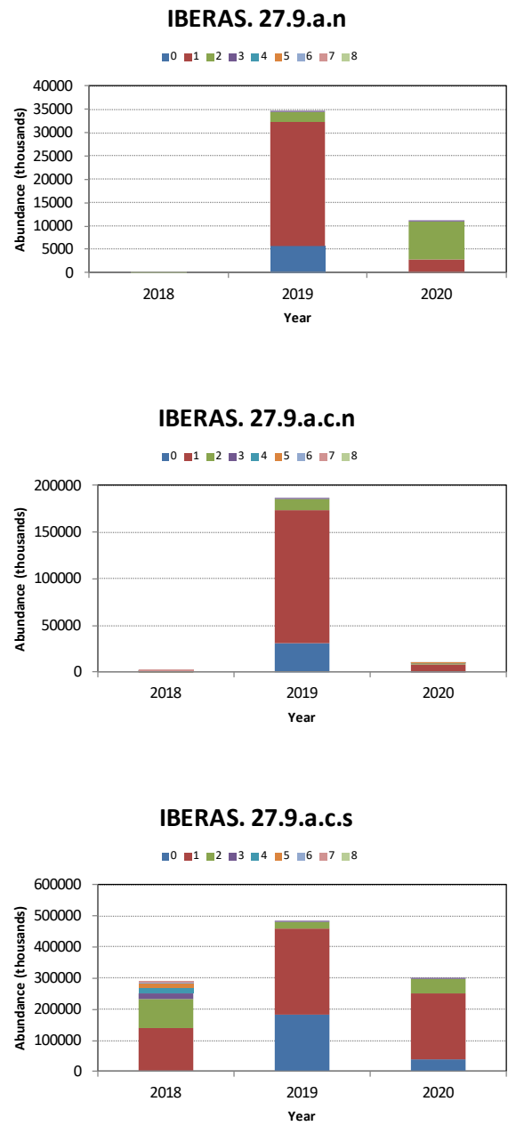
Figure 3.2.22. IBERAS Autumn acoustic-trawl survey series. Age structure of the chub mackerel estimated population (in thousands).
