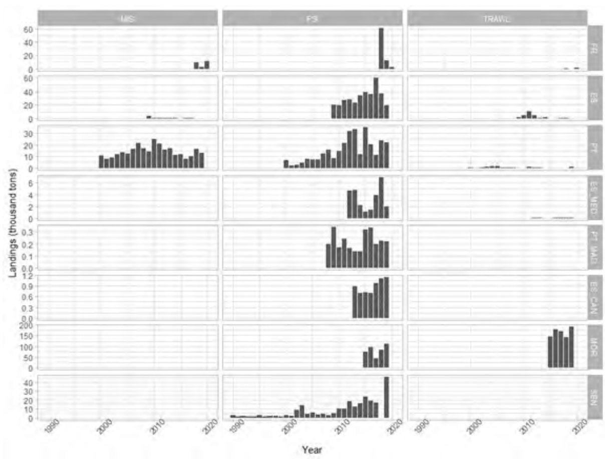
Figure 2.2.3. Chub mackerel landings (thousand tons) by Country/Region for the grouped gears MIS, PS and TRAWL (time period: 1990–2020). Fishing gears: MIS- Other fleets, PS- Purse-seiners, TRAWL- Trawlers.
