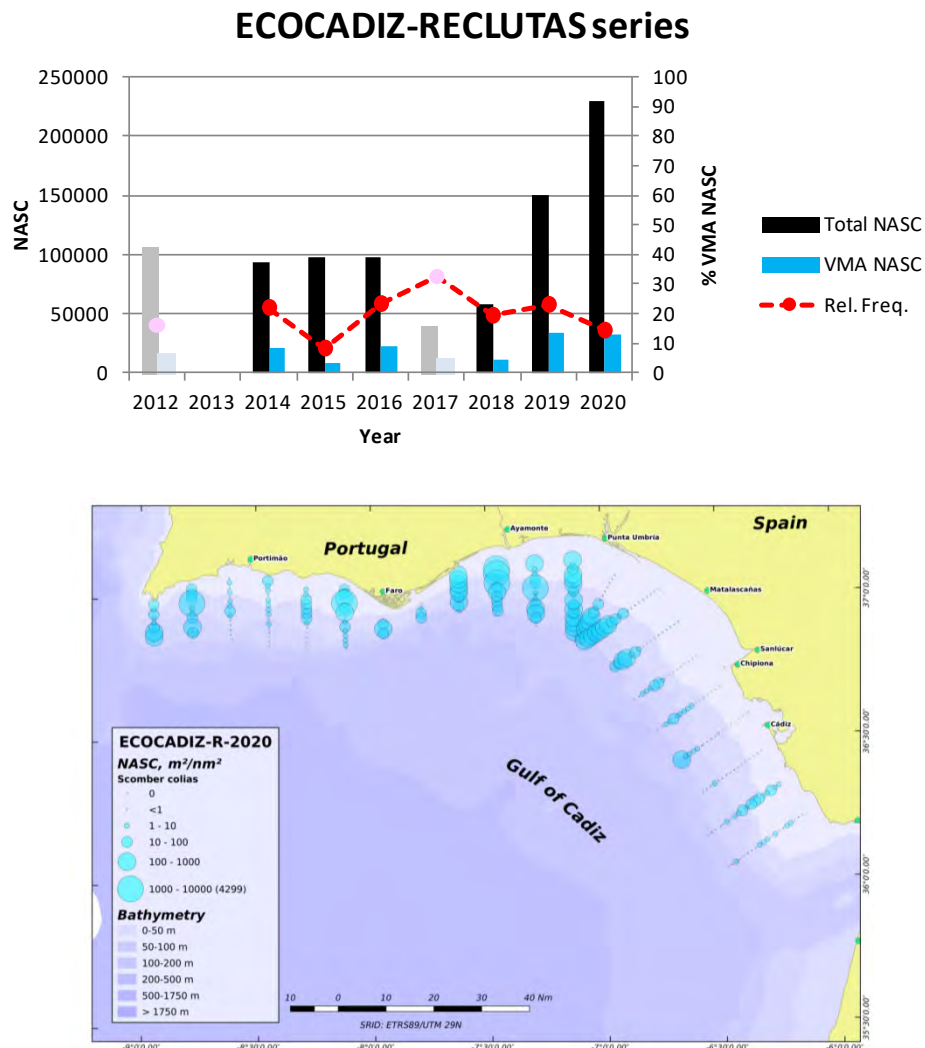
Figure 3.2.17. ECOCADIZ-RECLUTAS Autumn acoustic-trawl survey series. ICES subdivisions 27.9.a.s.a and 27.9.a.s.c (Gulf of Cadiz). Upper panel: time-series of estimates of acoustic density (NASC estimates; m 2 nm -2 ). The 2012 survey only covered the Spanish waters whereas the 2017 survey only covered the Spanish eastern waters because of a serious breakdown of the vessel's propulsion system. Bottom panel: distribution of the acoustic densities (NASC, m 2 nm -2 ) for chub mackerel in 2020 (source: Ramos and Carrera presentation during the WK; abstract without figures available in Annex 4).
