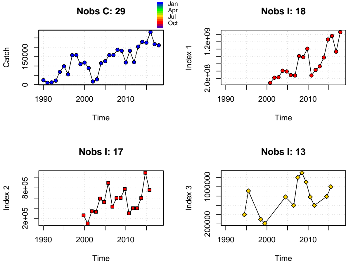
Figure 2: Data input summary. Top left: chub mackerel catches in tonnes. Top right: Amir Moulay Abdellah acoustic estimates (autumn). Bottom left: Nansen acoustic estimates (autumn). Bottom right: Atlantida acoustic estimates (summer).
