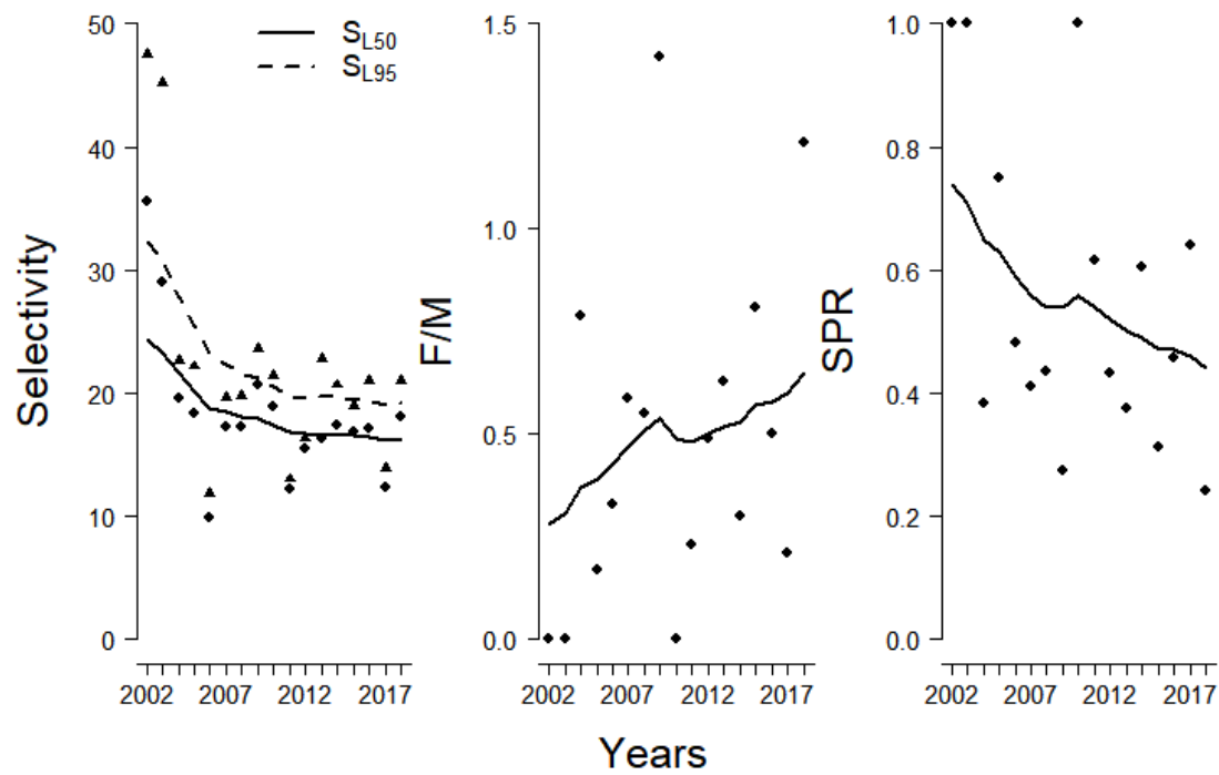
Figure 7.3.2.6.3. Moroccan central and southern chub mackerel stock: Estimated values for SPR, SL50, SL95 and F/M for scenario 1; the black line corresponds to the smoother line to the estimated points.
