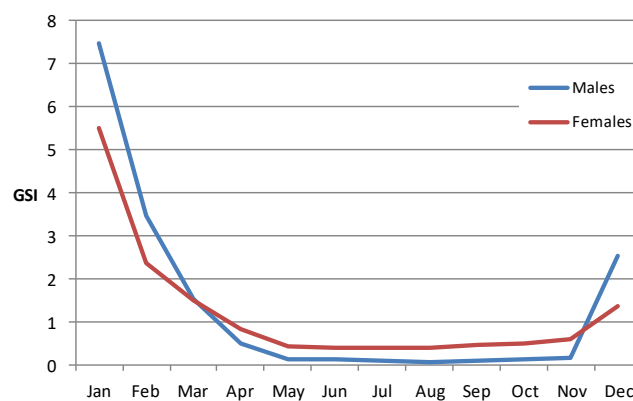
Figure 7. Monthly averaged GSI by sex (2013-2019)
