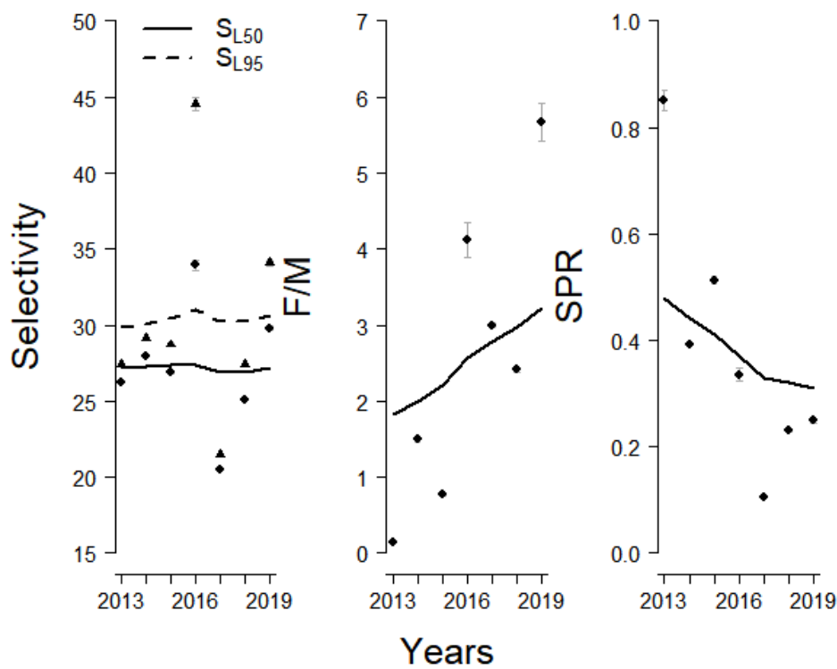
Figure 7.3.2.1.3. Cantabrian Sea (27.8.c) chub mackerel: Estimated values for SPR, S_{L50} , S_{L95} and F/M for scenario 1; the black line corresponds to the smoother line to the estimated points.
