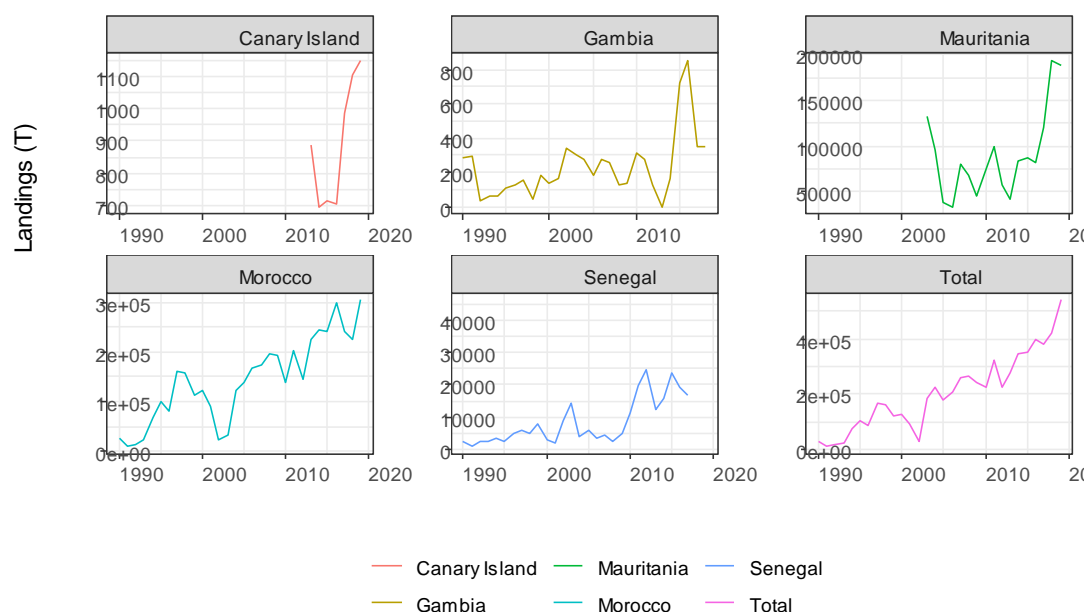
Figure 2.2.2. Annual evolution of chub mackerel landings (tons) in the NW African waters (time period: 1990–2019).
