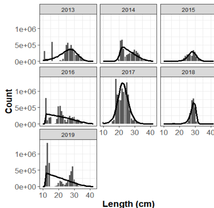
Figure 7.3.2.3.1. Chub mackerel in Mediterranean Sea – Catalan Sea: Length composition distributions for chub mackerel landings (bars) and LBSPR model fit (solid black line).
