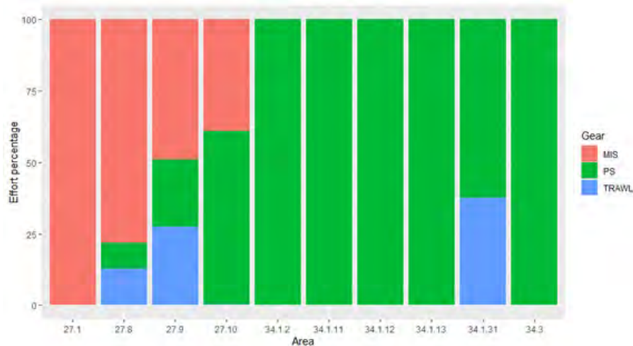
Figure 2.4.1. Fishing effort per gear in each area, using annual weighted mean values. Fishing gears: MIS- Other fleets, PS- Purse-seiners, TRAWL- Trawlers.
