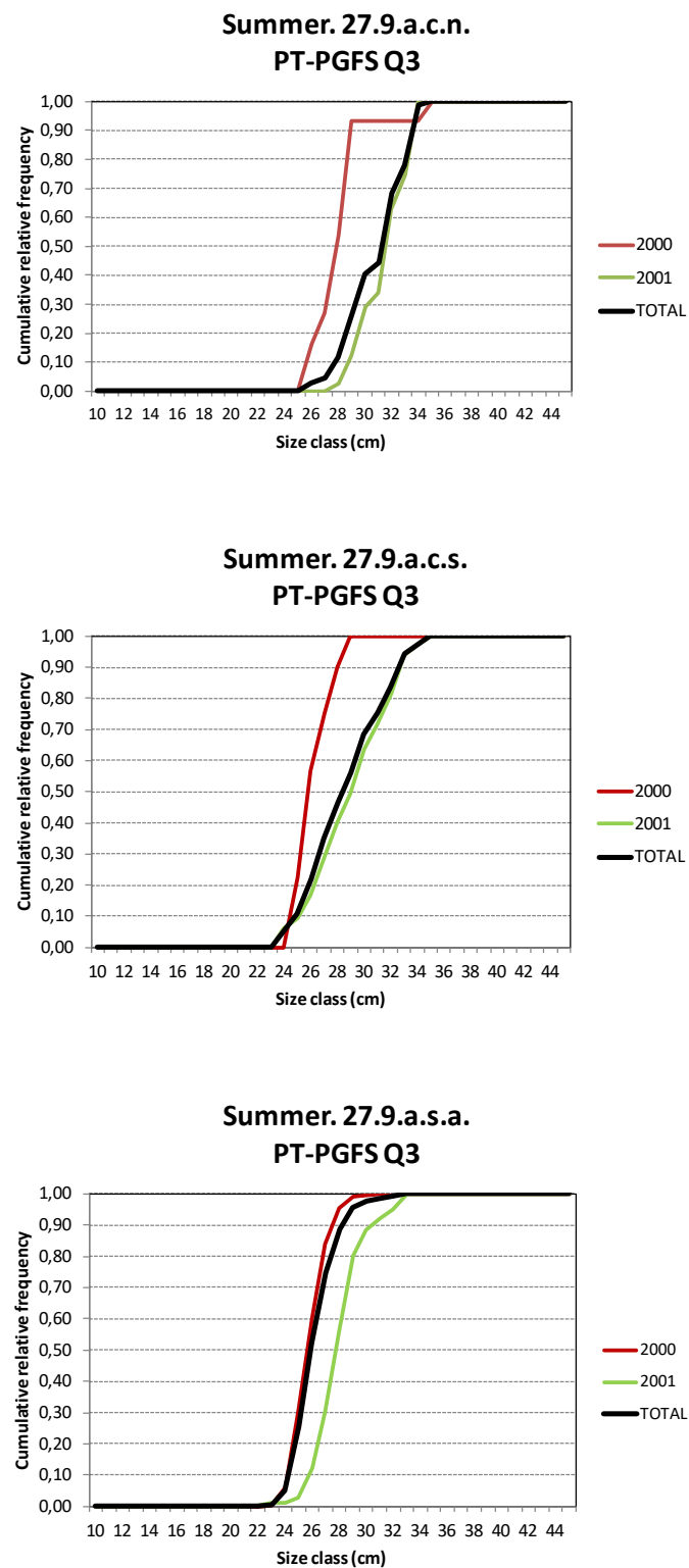
Figure 3.2.10. PT-PGFS Q3 (3rd quarter) Summer bottom-trawl survey series. Cumulative size relative frequencies for chub mackerel by ICES subdivision. Total refers to pooled data for the available time-series.
