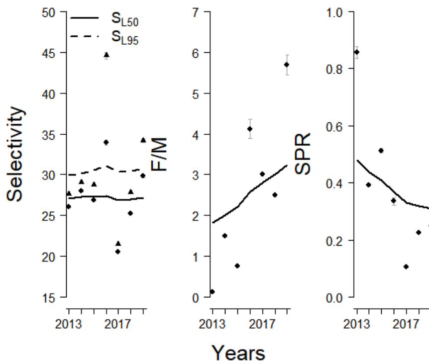
Figure 7.3.2.1.9. Cantabrian Sea (27.8.c) chub mackerel discards: Estimated values for SPR, SL50, SL95 and F/M for discards and scenario 1; the black line corresponds to the smoother line to the estimated points.
