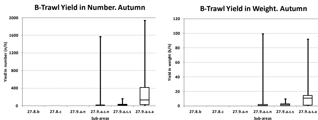
Figure 3.2.26. Autumn bottom-trawl survey series. Box-plot of regional estimates of chub mackerel relative abundance (n/haul) and biomass (kg/haul). Outliers not shown. Years 2000–2011, 2013–2018.
