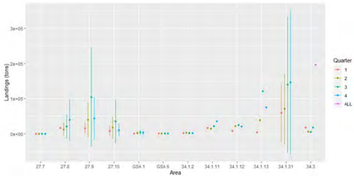
Figure 2.2.8. Quarter variability of the chub mackerel landings within area (point – mean value; vertical lines – mean \pm sd).
