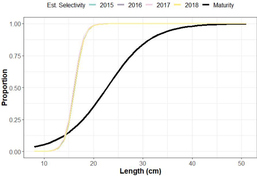
Figure 7.3.2.7.2. Moroccan northern chub mackerel: Specified maturity and estimated selectivity-at-length.
