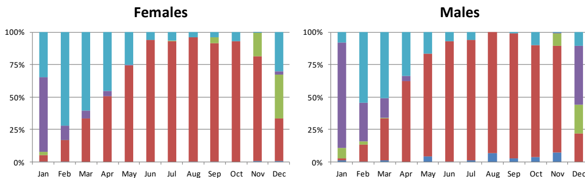
Figure 6. Monthly proportions of maturity stages by sex (2013-2019)
