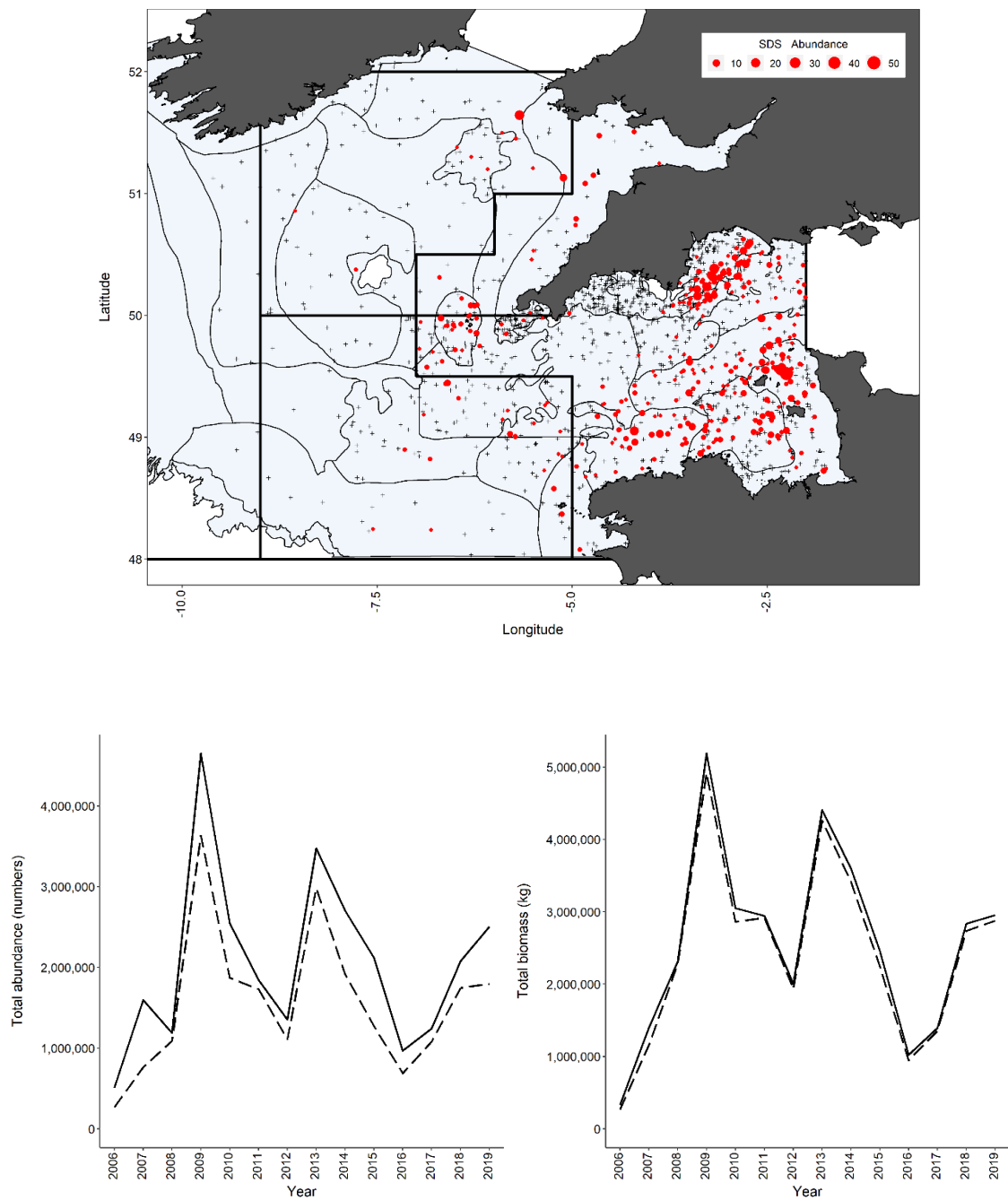
Figure 21.8. Survey grid of the Q1SWECOS survey (2006–2019) indicating the distribution and relative abundance of Mustelus spp. (top), and the total abundance (numbers) and total biomass (kg) for Mustelus spp (bottom). Continuous line relates to all specimens, dashed line relates to individuals \geq 50 cm total length. Source: Silva et al. (2020 WD).
