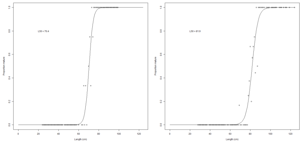
Figure 21.15. Smooth-hounds in the Northeast Atlantic. Maturity ogive for male (n = 237; L 50 = 70.4 = cm L 7 ) and female (n = 248; L 50 = 81.9 cm L 7 ) M. asterias . Source: McCully Phillips and Ellis (2015).
