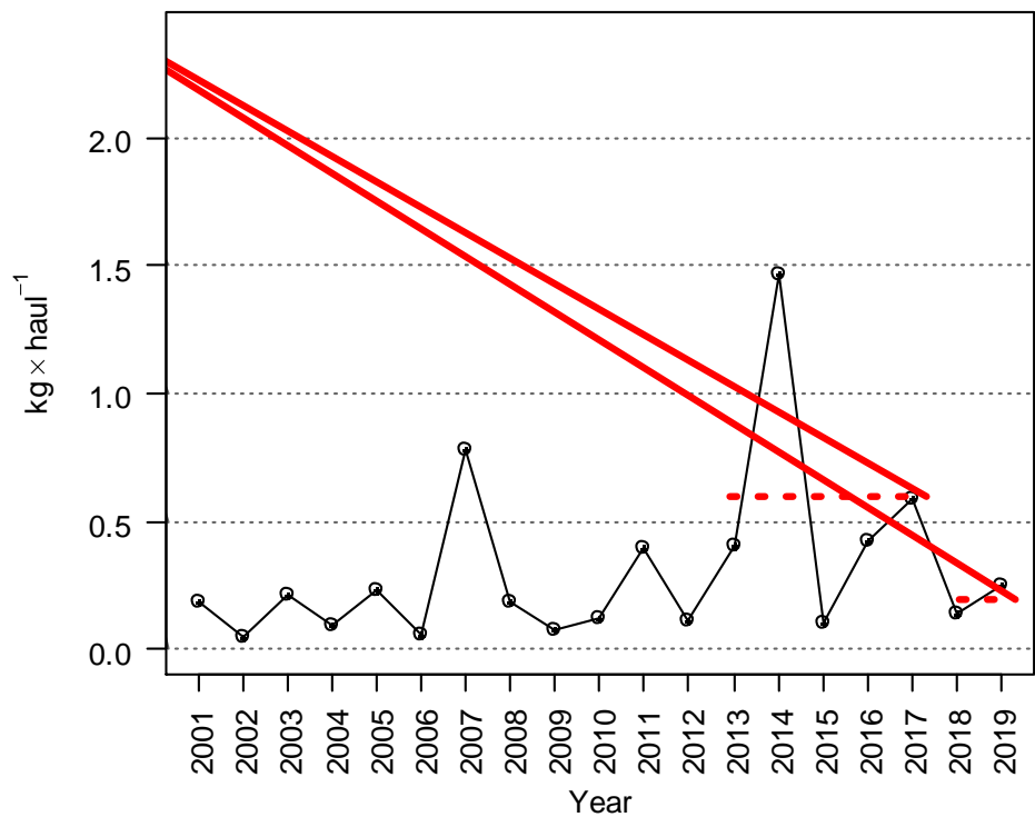
Figure 4.3. Evolution in kitefin shark biomass index in Porcupine surveys (2001–2019). Dotted red lines compare mean stratified biomass in the last two years (2018–2019) with the five previous years (2013–2017). Source: Ruiz-Pico et al. (2020 WD02).
