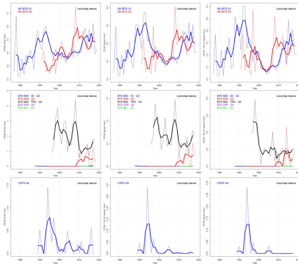
Figure 15.6.2. Demersal elasmobranchs in the North Sea, Skagerrak, Kattegat and eastern Channel. Leucoraja naevus . Abundance index ( \text{n. hr}^{-1} ), biomass index ( \text{kg hr}^{-1} ) and exploitable biomass ( \text{kg hr}^{-1} ), including their three year running means, during the North Sea IBTS (in roundfish areas 1–7), BTS, and CGFS surveys in the years 1977–2018. Data extracted from the DATRAS database (selected for CPUE per length per haul) on 12 June 2019.
