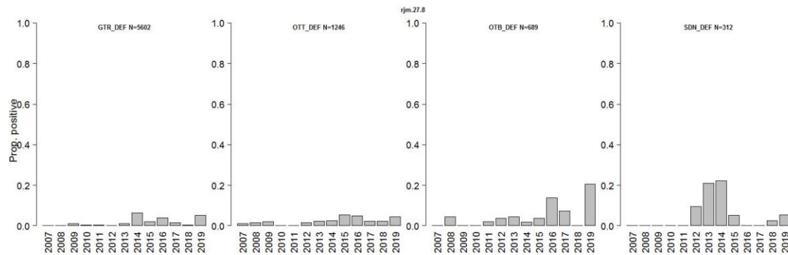
Figure 19.19. Skates in the Bay of Biscay and Iberian Waters. Raja montagui in Subarea 8 (rjm.27.8). Occurrence indicators from the French on-board observer trips carried out in application of EU data collection programmes in divisions 8.abd. N: total number of fishing operations observed for the métier from 2008 to 2019.
