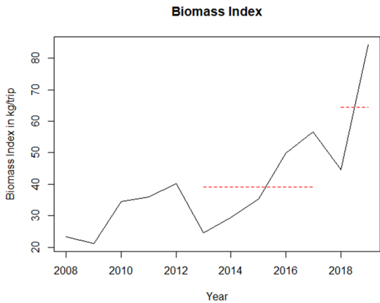
Figure 19.4c. Skates in the Bay of Biscay and Iberian Waters. Annual standardized CPUE estimates (kg trip -1 ) of R. brachyura in the Division 9.a of the Portuguese Polyvalent fleet for the period 2008–2019.
