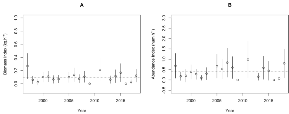
Figure 19.11b. Skates in the Bay of Biscay and Iberian Waters. Leucoraja naevus A) biomass index (kg hour -1 ) and B) abundance (ind.hour -1 ) on PT-CTS (UWTV (FU 28-29) from 1997 to 2018. Dashed line represents the mean annual abundance for the considered period.
