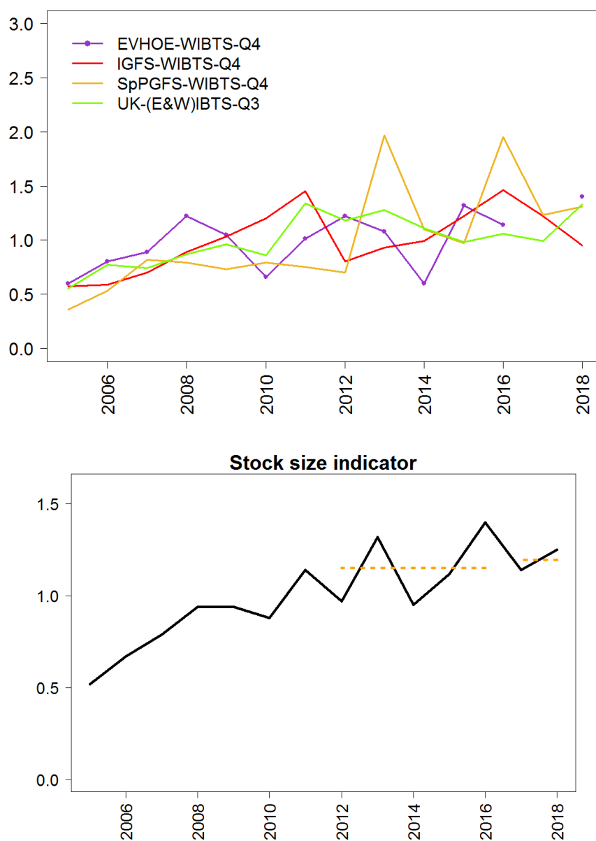
Figure 25.6a. Catsharks (Scyliorhinidae) in the Northeast Atlantic. Scyliorhinus canicula in the Celtic Seas Ecoregion. Standardised survey indices from four surveys IGFS-WIBTS-Q4, Spanish Porcupine Bank survey SpPGFS-WIBTS-Q4, UK-(E&W)-BTS-Q3, EVHOE-WIBTS-Q4 (top) and overall stock size indicator (bottom) for the time period 2005–2018. Dotted lines indicate the average of the last two years and the average catch for the preceding five years.
