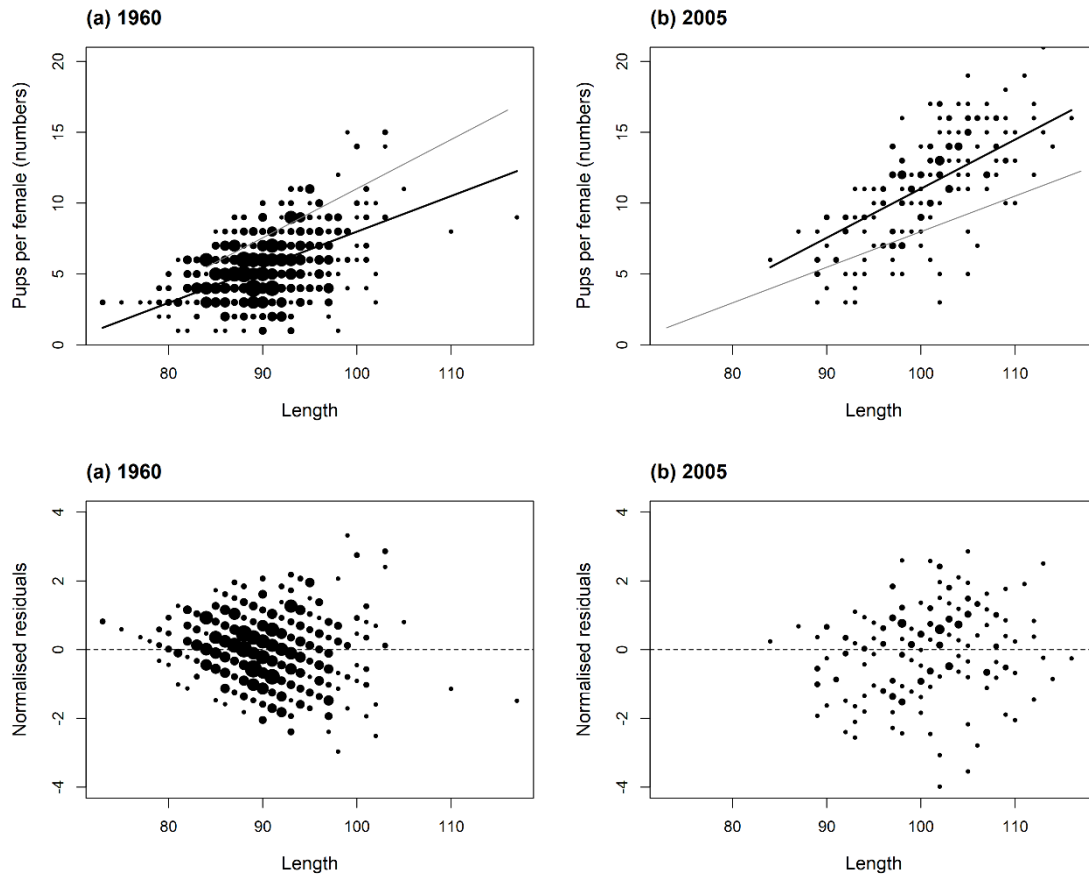
Figure 2.25a. Northeast Atlantic spurdog. C_{SQ} assessment. Fit to fecundity data from two periods (top row) (a) 1960 and (b) 2005, with associated normalised residuals ( \varepsilon_{fec,k,y} in Stock Annex equation 11b) (bottom row). For the top plots, the heavy black lines reflect the model estimates for the given points, while the light grey ones, reflecting the model estimates for the points in the adjacent plot, are given for comparison. For all plots, the diameter of each point is proportional to \sqrt{n} , where n is the number of samples with the same number of pups for a given length.
