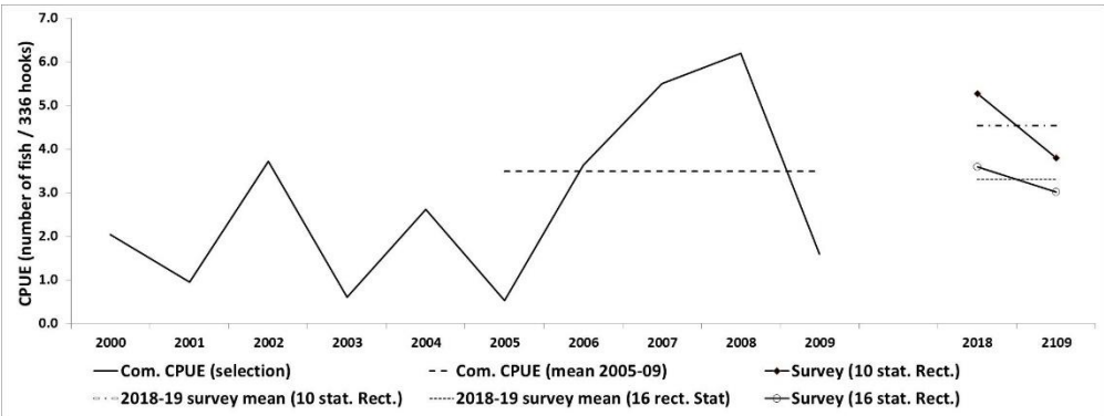
Figure 6.9. 2018-2019 CPUE (in number of porbeagles per long line set of 336 hooks) of the 2018–2019 survey and of a 2000–2009 commercial CPUE series built with selections to make it comparable to the survey indices (from Biais, 2019). Two survey CPUEs are shown, one for the entire survey area including 16 statistical rectangles and one including 10 statistical rectangles, which excluded those rectangles with mean CPUEs of less than 1 fish/336 hooks in 2018 or less than 1.5 fish/336 hooks in 2019.
