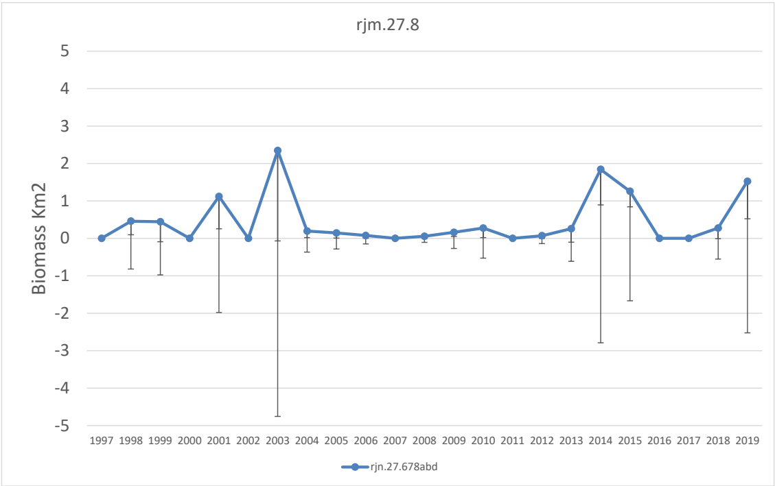
Figure 19.6c. Skates in the Bay of Biscay and Iberian Waters. Biomass index ( \text{kg km}^{-2} ) of R. montagui in the Subarea 8. Abundance and biomass are raised to the total area ( \text{km}^2 ) surveyed (swept area method) but should be considered relative and not absolute estimates.
