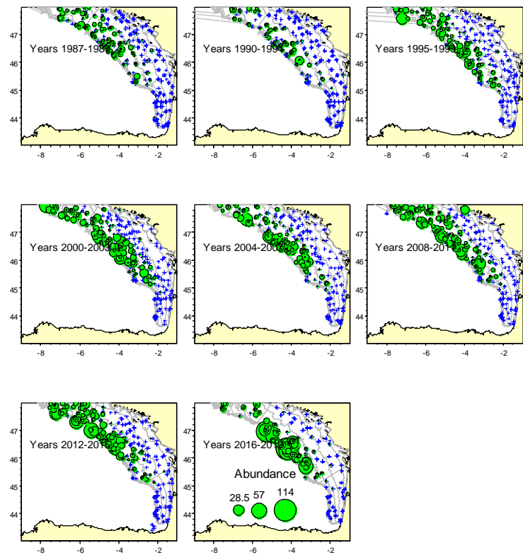
Figure 19.5a. Skates in the Bay of Biscay and Iberian Waters. Spatial distribution of L. naevus (catches in number per haul) by groups of four years from the EVHOE survey in the Bay of Biscay.
