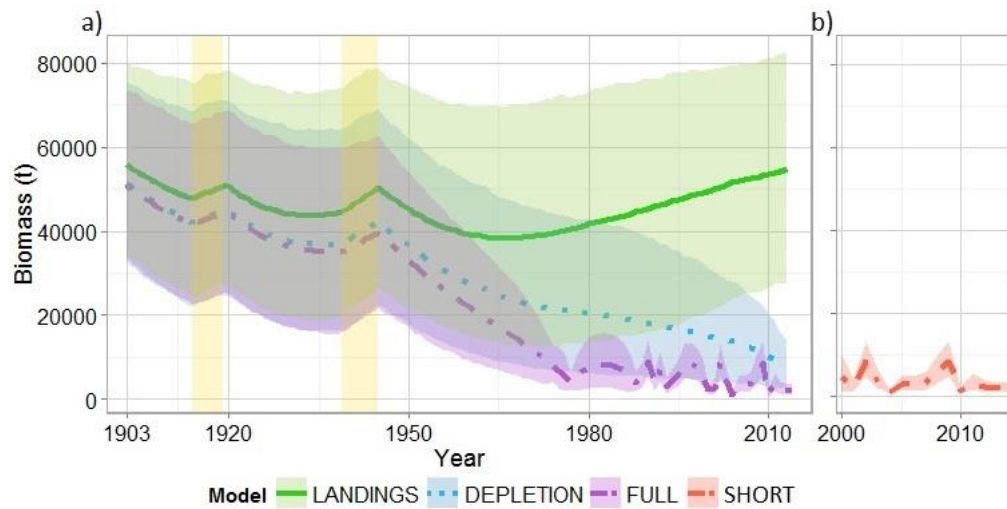
Figure 19.15. Skates in the Bay of Biscay and Iberian Waters. a) Estimated biomass trajectories for R. clavata in the Bay of Biscay for model runs using different data series. LANDINGS: landings only; DEPLETION: landings and final year depletion rate; FULL: landings and biomass index for the years 1973–2013. Coloured areas: credible intervals between 2.5 and 97.5 percentiles. Vertical rectangles: World War I and II periods. b) Estimated biomass trajectories for R. clavata in the Bay of Biscay by using only catches and biomass index time series from 2000 to 2013 (SHORT run).
