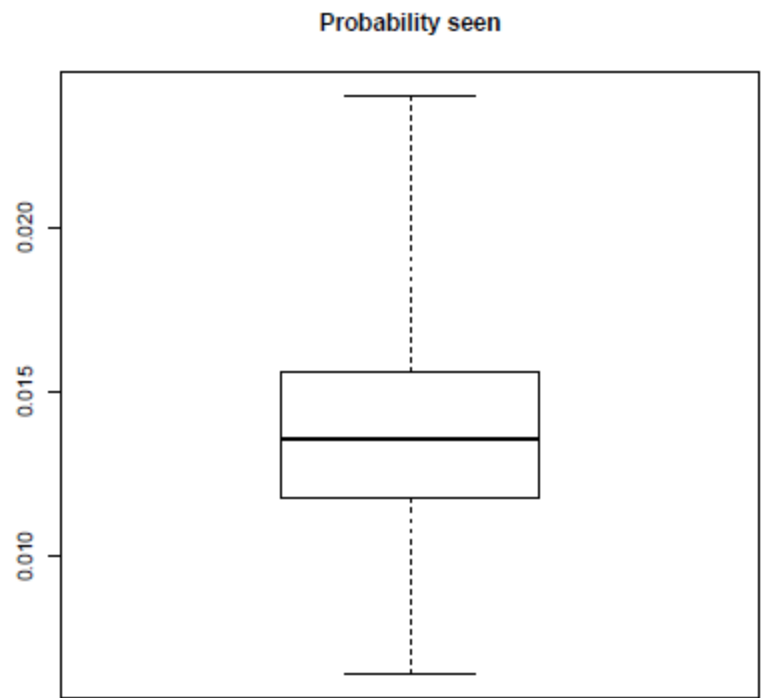
Figure 10.14. Tope in the Northeast Atlantic. Individual capture probability posterior.
