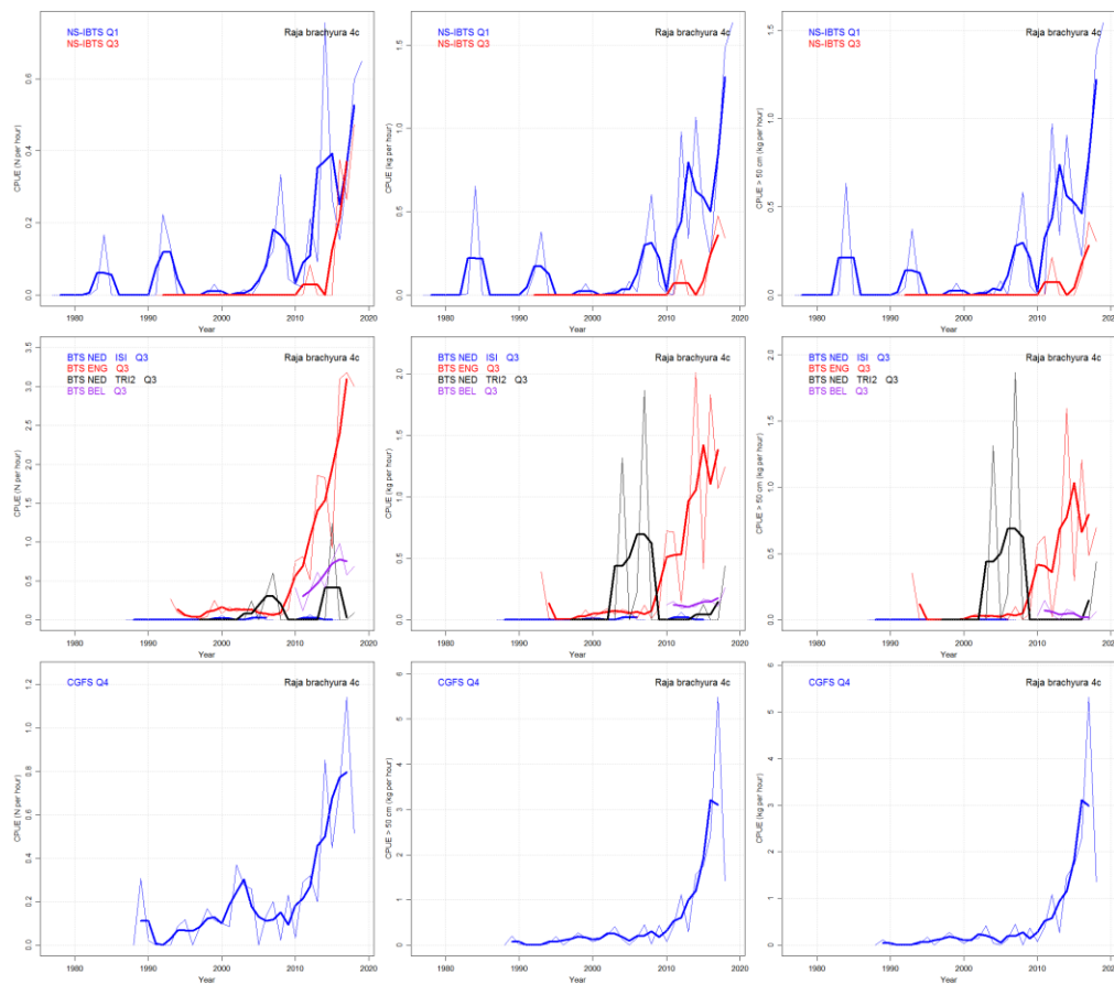
Figure 15.6.7. Demersal elasmobranchs in the North Sea, Skagerrak, Kattegat and eastern Channel. Raja brachyura 4.c. Abundance index ( \text{n. hr}^{-1} ), biomass index ( \text{kg hr}^{-1} ) and exploitable biomass ( \text{kg hr}^{-1} ), including their three year running means, during the North Sea IBTS (in roundfish areas 1–7), BTS, and CGFS surveys in the years 1977–2018. Data extracted from the DATRAS database (selected for CPUE per length per haul) on 12 June 2019.
