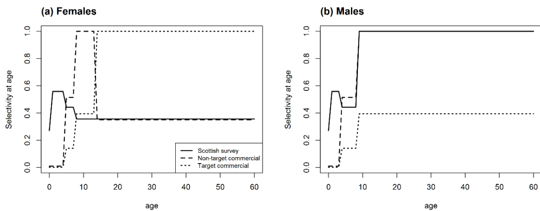
Figure 2.26b. Northeast Atlantic spurdog. H_{RSQ} assessment. Estimated selectivity-at-age curves for the base case run for (a) females and (b) males. The two commercial fleets considered have non-target (Scottish) and target (England & Wales) selectivity, which differ by sex because of the life-history parameters for males and females (Table 2.6). The survey selectivity relies on Scottish survey data.
