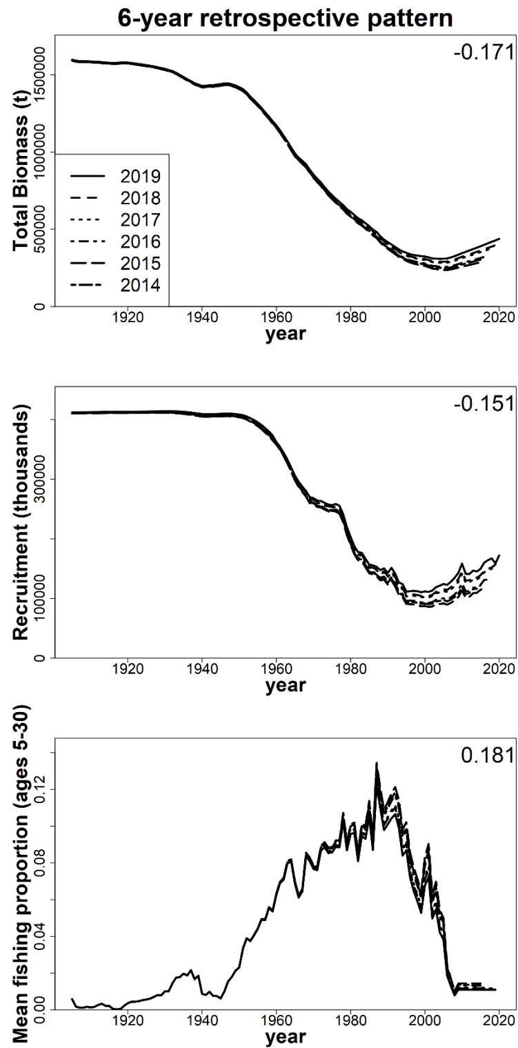
Figure 2.28b. Northeast Atlantic spurdog. HR_{SQ} assessment. Six-year retrospective plots (omitting probability intervals for clarity; the model was re-run, each time omitting a further year in the data).
