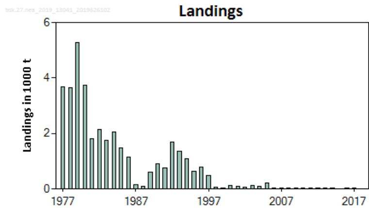
Figure 7.1. Basking shark in the Northeast Atlantic. Total landings (1000 t) of basking sharks in ICES subareas 1–14 from 1977–2018, since 2013: < 1 t landed.
