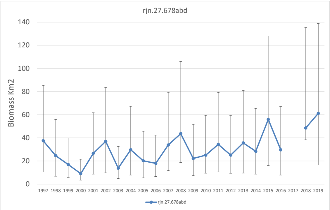
Figure 19.6a. Skates in the Bay of Biscay and Iberian Waters. Biomass indices 1987 index ( \text{kg km}^{-2} ) of L. naevus from the EVHOE survey 1997–2019 in divisions 8.abd.
