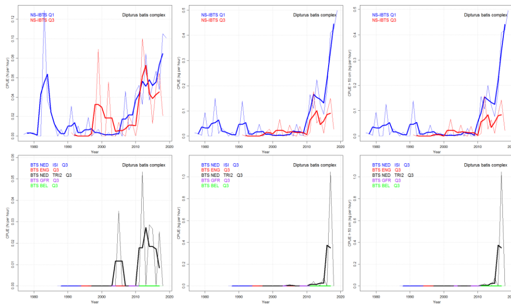
Figure 15.6.5. Demersal elasmobranchs in the North Sea, Skagerrak, Kattegat and eastern Channel. 'Common skate complex'. Abundance index ( \text{n. hr}^{-1} ), biomass index ( \text{kg hr}^{-1} ) and exploitable biomass ( \text{kg hr}^{-1} ), including their three year running means, during the North Sea IBTS (in roundfish areas 1–7), BTS, and CGFS surveys in the years 1977–2018. Data extracted from the DATRAS database (selected for CPUE per length per haul) on 12 June 2019.
