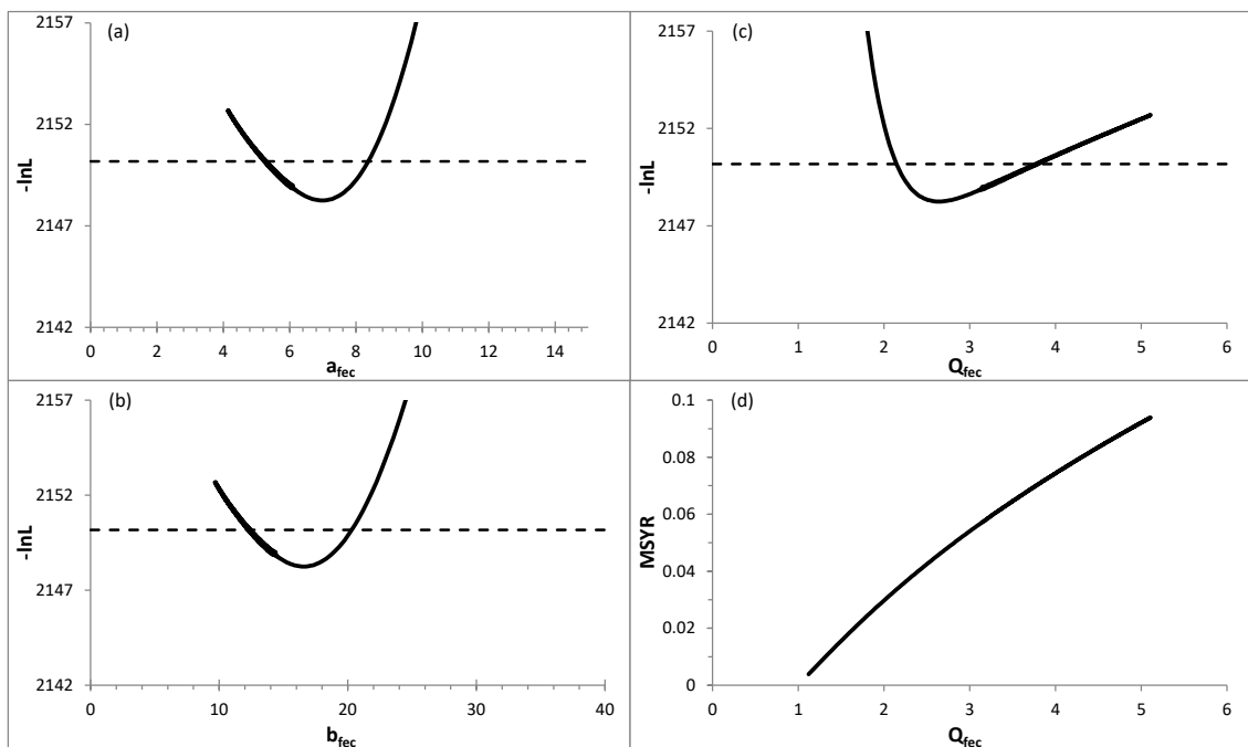
Figure 2.21a. Northeast Atlantic spurdog. CSQ assessment. Negative log-likelihood ( -\ln L ) for a range of (a) a_{fec} and (b) b_{fec} values, with (c) corresponding Q_{fec} . Plot (d) shows MSYR ( \text{MSY}/B_{\text{MSY}} ) vs. Q_{fec} . Using the likelihood ratio criterion, the hashed line in plots (a)–(c) indicate the minimum -\ln L value + 1.92, corresponding to 95% probability intervals for the corresponding parameters for values below the line.
