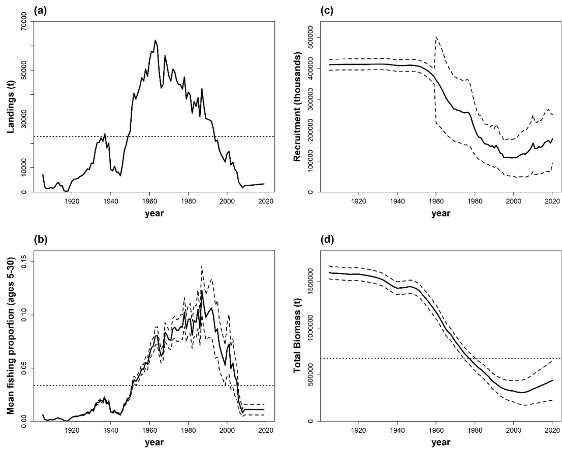
Figure 2.32b. Northeast Atlantic spurdog. HR SQ assessment. Summary four-plot for the base-case, showing long-term trends in landings (tons; dotted horizontal line = MSY = 22\,874\text{ t} ), recruitment (thousands of pups), mean fishing proportion (average ages 5–30; dotted horizontal line = F_{prop,MSY} = 0.033 ) and total biomass (tons; dotted horizontal line = MSY\ B_{trigger} = 677\,830\text{ t} ). Hashed lines reflect estimates of precision ( \pm 2 standard deviations).
