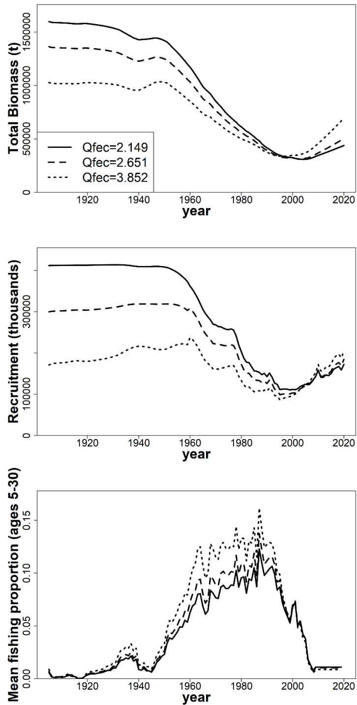
Figure 2.29b. Northeast Atlantic spurdog. HR SD assessment. A sensitivity analysis of the parameter that determines the extent of density-dependence in pup production ( Q_{fec} ). Three alternative values are considered, related to the smallest, optimum (in terms of lowest -\ln L ) and largest value of Q_{fec} below the hashed line in Figure 2.21c (respectively 2.149 [base case], 2.651 and 3.852).
