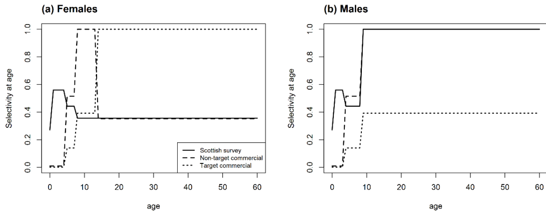
Figure 2.26a. Northeast Atlantic spurdog. C_{SQ} assessment. Estimated selectivity-at-age curves for the base case run for (a) females and (b) males. The two commercial fleets considered have non-target (Scottish) and target (England & Wales) selectivity, which differ by sex because of the life-history parameters for males and females (Table 2.6). The survey selectivity relies on Scottish survey data.
