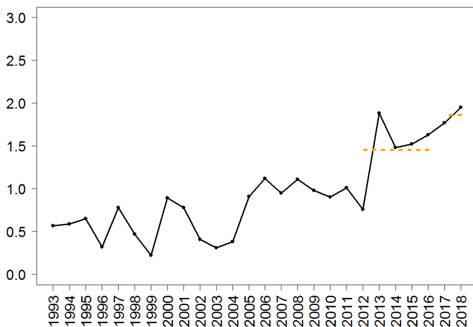
Figure 25.8b. Catsharks (Scyliorhinidae) in the Northeast Atlantic. Scyliorhinus canicula in the Atlantic Iberian waters (divisions 8.c and 9.a). Overall stock size indicator combined for these surveys (bottom). Dotted lines indicate the average of the last two years and the average catch for the preceding five years.
