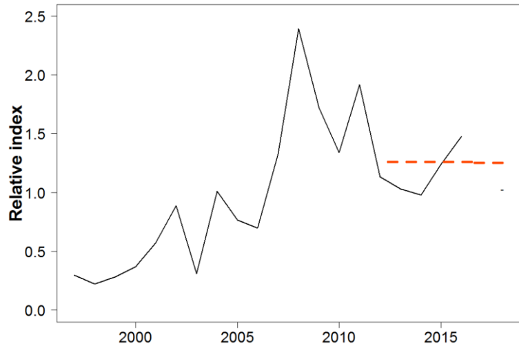
Figure 25.7. Catsharks (Scyliorhinidae) in the Northeast Atlantic. Trends in the stock size of Scyliorhinus canicula in the Bay of Biscay (ICES divisions 8.a-b, d), as estimated from the EVHOE survey.
