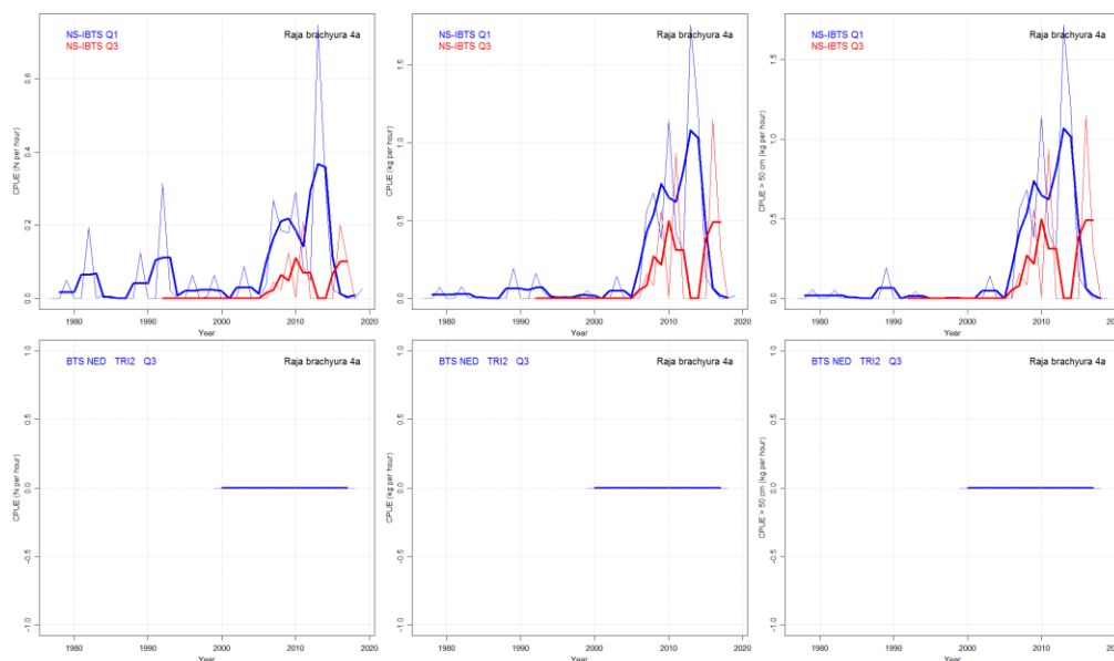
Figure 15.6.6. Demersal elasmobranchs in the North Sea, Skagerrak, Kattegat and eastern Channel. Raja brachyura in 4.a. Abundance index ( \text{n. hr}^{-1} ), biomass index ( \text{kg hr}^{-1} ) and exploitable biomass ( \text{kg hr}^{-1} ), including their three year running means, during the North Sea IBTS (in roundfish areas 1–7), BTS, and CGFS surveys in the years 1977–2018. Data extracted from the DATRAS database (selected for CPUE per length per haul) on 12 June 2019.
