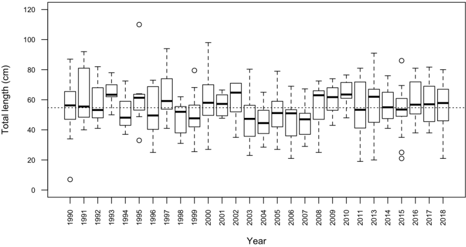
Figure 19.10c. Skates in the Bay of Biscay and Iberian Waters. Total length variation of Raja clavata , by year on PtGFS-WIBTS-Q4 (dashed line represents the mean annual length for 1990–2018).
