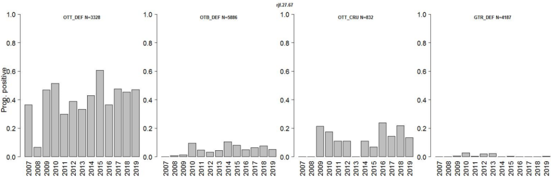
Figure 18.2 Skates and rays in the Celtic Seas. Temporal trends in the proportion of hauls encountering RJF.27.67, based on French on-board observer trips carried out in application of EU data collection programmes.
