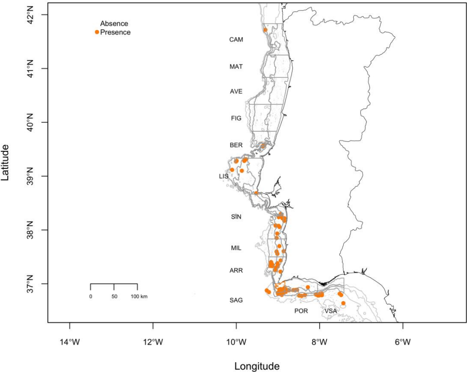
Figure 19.11a. Skates in the Bay of Biscay and Iberian Waters. Leucoraja naevus distribution from 1981 to 2018 in the Portuguese Autumn Groundfish Surveys (PtGFS-WIBTS-Q4), and Portuguese crustacean surveys/ Nephrops TV surveys (PT-CTS (UWTV (FU 28-29)).
