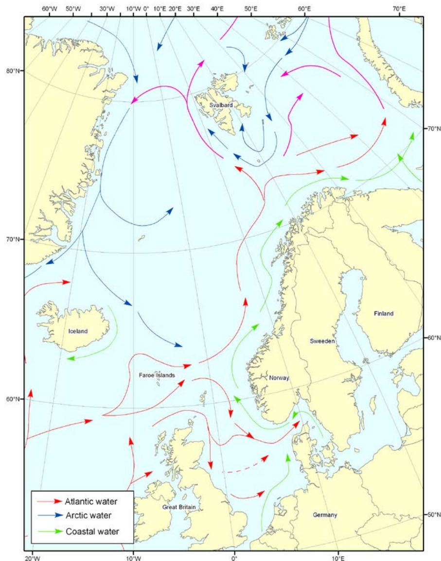
Figure A1-3. Prevailing ocean currents in the Northeast Atlantic. Map from Norwegian Institute of Marine Research (IMR).
