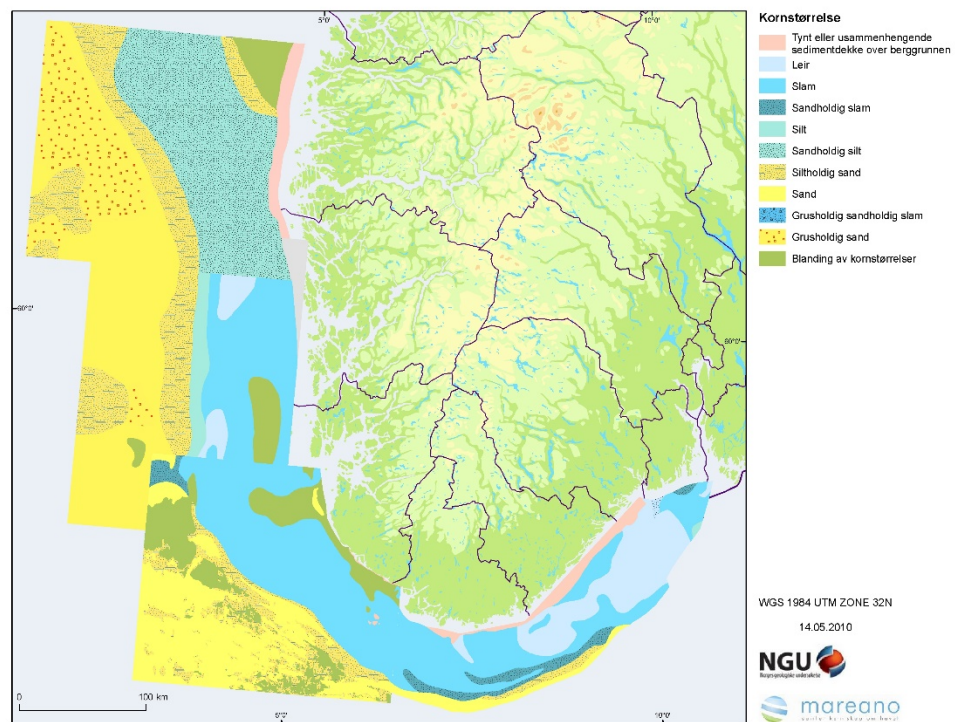
Figure A1-1. Sediment map of the Norwegian Deep and Skagerrak. Map from https://mareano.no .
