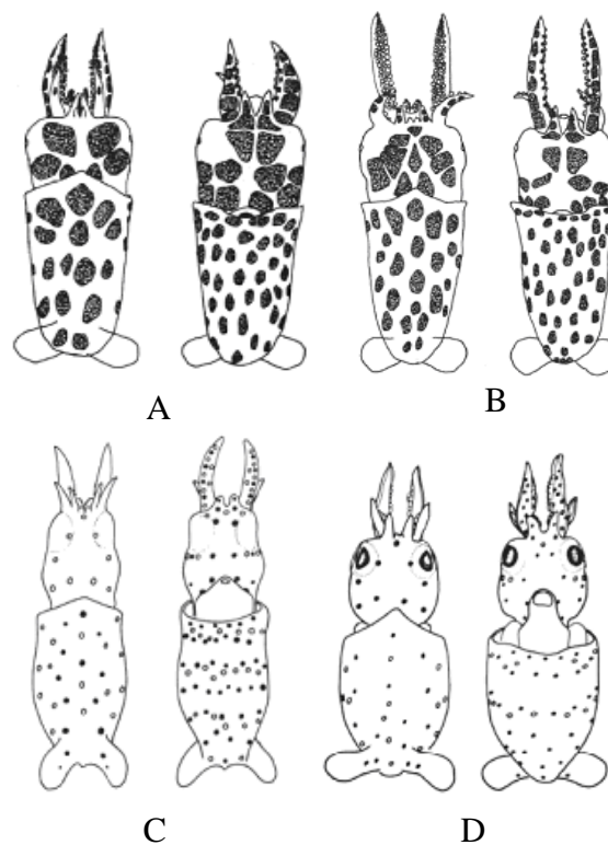
Figure 5.12. Loliginidae, dorsal (left) and ventral (right) views: Loligo vulgaris , 3.1 mm ML (A); Loligo forbesii , 3.7 mm ML (B); Alloteuthis media , live hatchlings (C); and Alloteuthis subulata , 2.0 mm ML (D). A, B, and D from Sweeney et al. (1992); C from Fioroni (1965).
