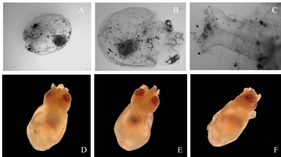
Figure 5.39. Rynchoteuthion type B: 2.04 mm ML paralarva (A, B) and detail of the proboscis of a 3.42 mm ML paralarva (C); dorsal (D), ventral (E) and lateral (F) views of a 3.0 mm ML paralarva. A–C from Moreno (2008).
