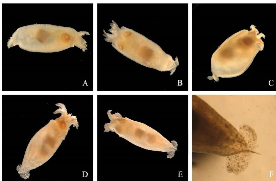
Figure 5.28. Onychoteuthidae paralarvae: lateral (A) and dorsal (B) views, 2.8 mm ML; lateral view (C), 2.9 mm ML; lateral (D) and dorsal (E) views, 3.0 mm ML; detail of the posterior mantle tip, 6.8 mm ML (F).
