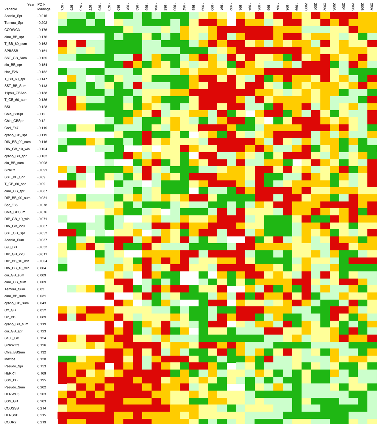
Figure 4.2.8. Traffic-light plot of the temporal development of the central Bothnian Sea time-series. Variables are transformed into quintiles, colour coded (green=low values; red=high values), and sorted in numerically descending order according to their loadings on the first principal component (PC1). Variable names are explained in Section 8 (Table 8.2).
