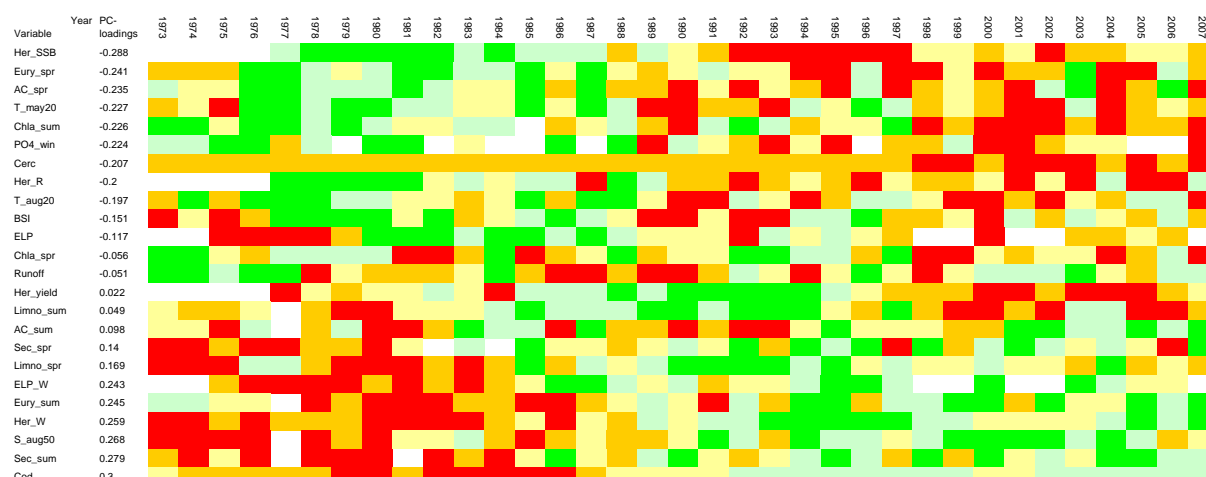
Figure 4.3.8. Traffic-light plot of the temporal development of the Gulf of Riga time-series. Variables are transformed into quintiles, colour coded (green = low values; red = high values), and sorted in numerically descending order according to their loadings on the first principal component (PC1). Variable names are explained in Section 8 (Table 8.3).
