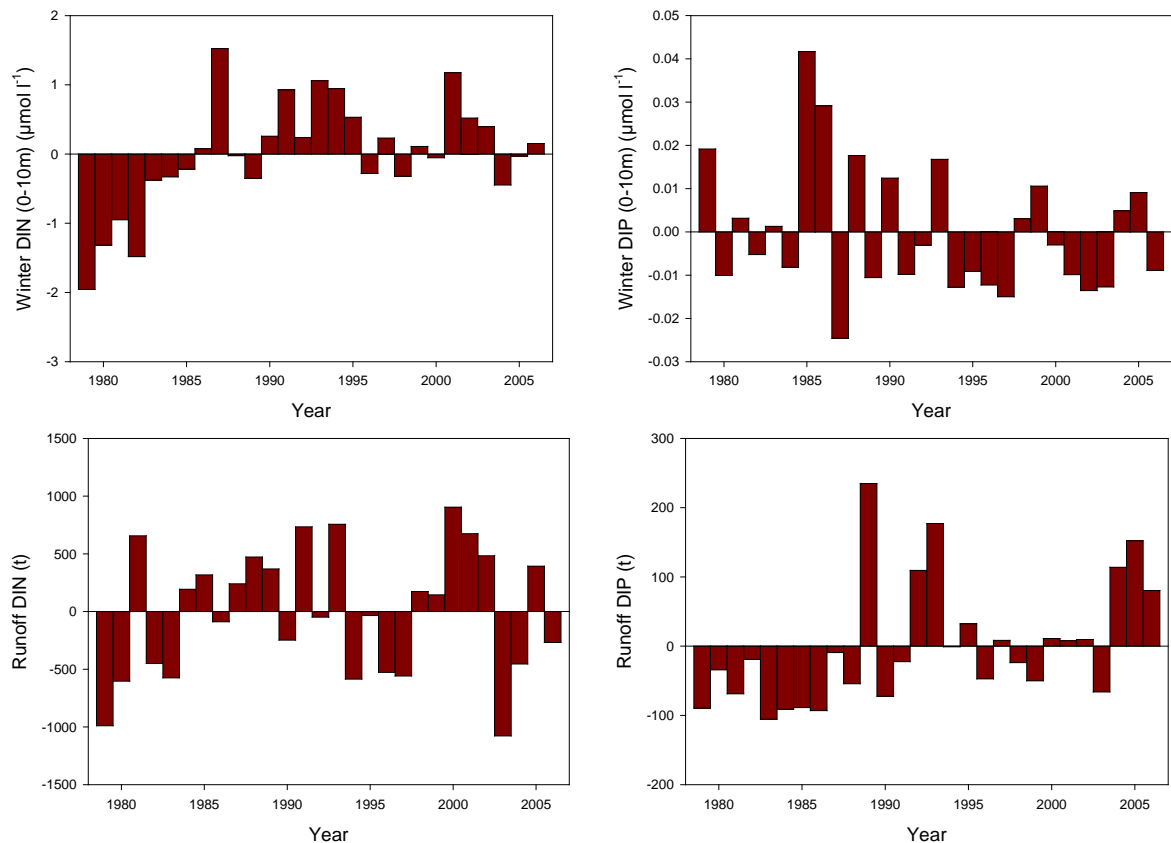
Figure 4.6.2. Long-term changes in nutrient concentrations in the Bothnian Bay. Anomalies of the overall mean for: (top) surface DIN (dissolved inorganic nitrogen; 6.53 \mu\text{mol l}^{-1} ) and DIP (dissolved inorganic phosphorus; 0.06 \mu\text{mol l}^{-1} ) in winter; and (bottom) total annual nutrient loads from run-off water from the western drainage basins, indicated by total DIN (3602 t) and DIP (215 t).
