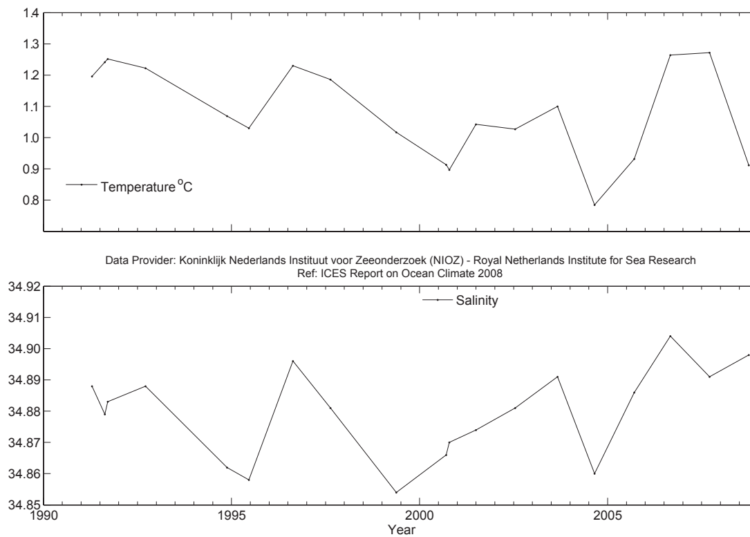
Figure 76. Area 3 – Icelandic Waters. Temperature at 1500–1800 m in the Iceland Sea (68°N 12.67°W).
