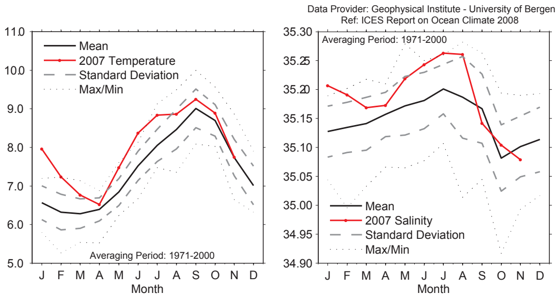
Figure 67. Norwegian Sea. 2007 monthly temperature (left panel) and salinity (right panel) at 50 m at Ocean Weather Station "Mike" (66°N 2°E). NOTE: No updates of monthly data are available for 2008.
