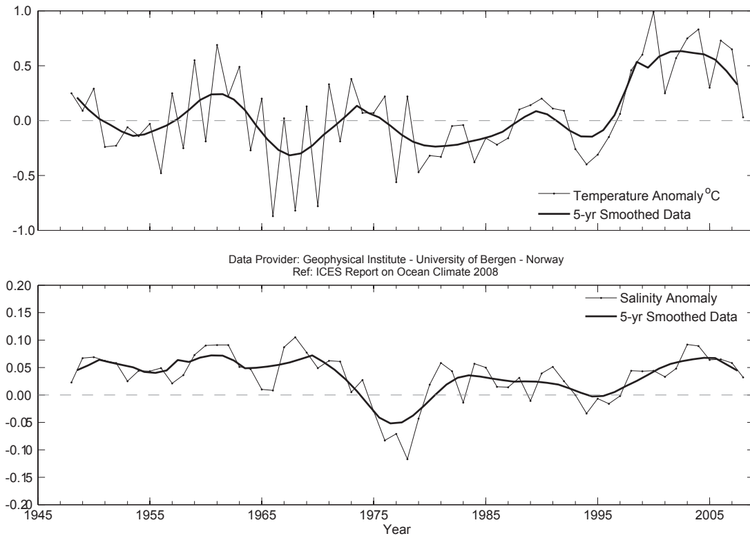
Figure 66. Area 10 – Norwegian Sea. Temperature anomaly (upper panel) and salinity anomaly (lower panel) at 50 m at Ocean Weather Station "Mike" (66°N 2°E).
