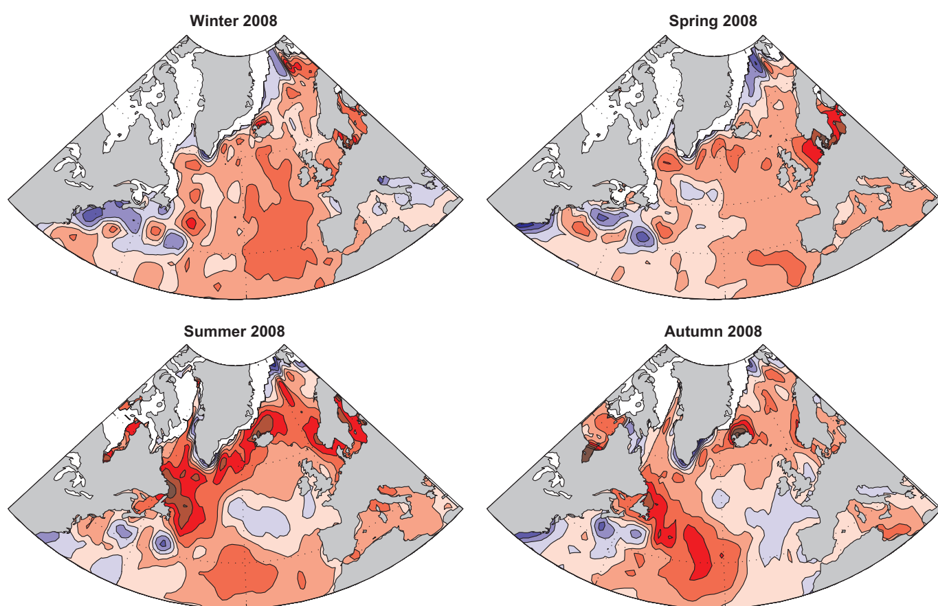
Figure 3. Maps of seasonal sea surface temperature anomalies (°C) over the North Atlantic for 2008 from the NOAA Optimum Interpolation SSTv2 dataset provided by the NOAA-CIRES Climate Diagnostics Center, US. The colour-coded temperature scale is the same in all panels. The anomaly is calculated with respect to normal conditions for 1971–2000. The data are produced on a one-degree grid from a combination of satellite and in situ temperature data. Regions with ice cover for >50% of the averaging period are left blank.
