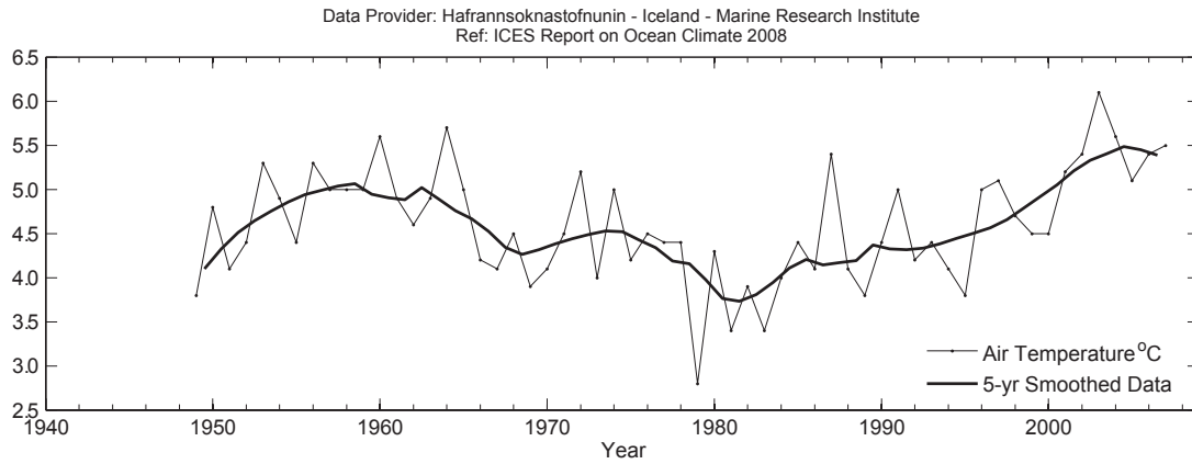
Figure 32. Area 3 – Icelandic waters. Mean annual air temperature at Reykjavík (upper panel) and Akureyri (lower panel).
