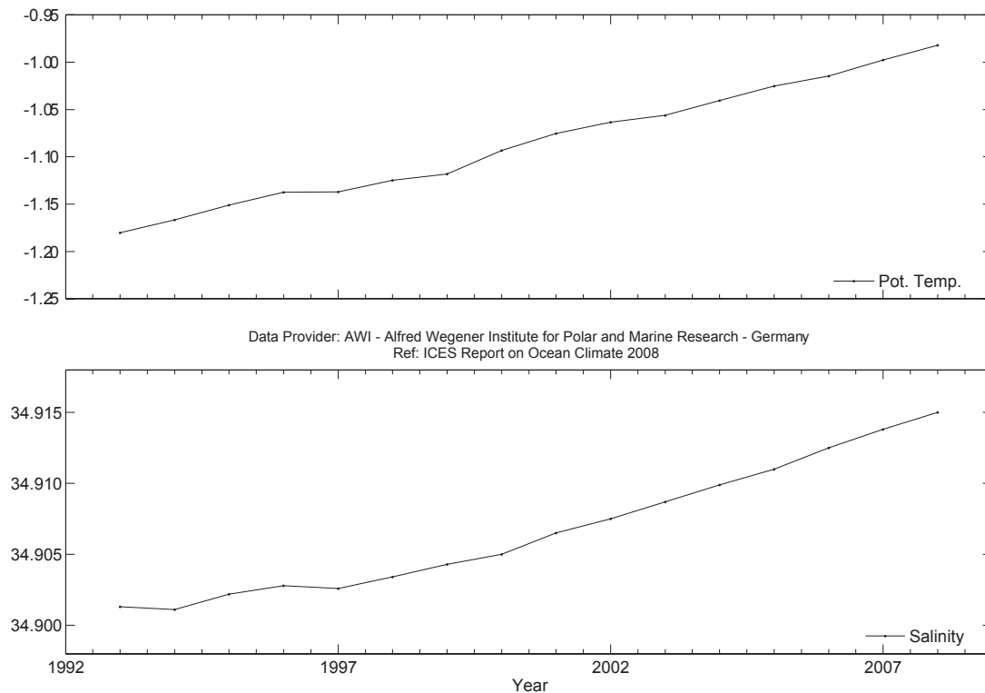
Figure 75. Area 12 – Greenland Sea and Fram Strait. Temperature (upper panel) and salinity (lower panel) at 3000 m in the Greenland Sea Section at 75°N.
