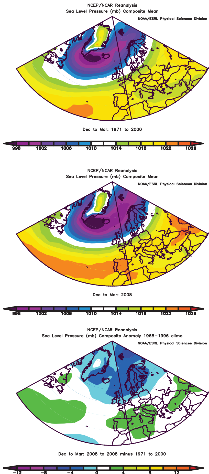
Figure 10. Winter (DJFM) sea level pressure (SLP) fields. Top panel: SLP averaged over 30 years (1971–2000). Middle panel: mean SLP in winter 2008 (December 2007, January–March 2008). Bottom panel: winter 2008 SLP anomaly – the difference between the top and middle panels. Images provided by the NOAA/ESRL Physical Sciences Division, Boulder, Colorado (available online at http://www.cdc.noaa.gov/ ).
