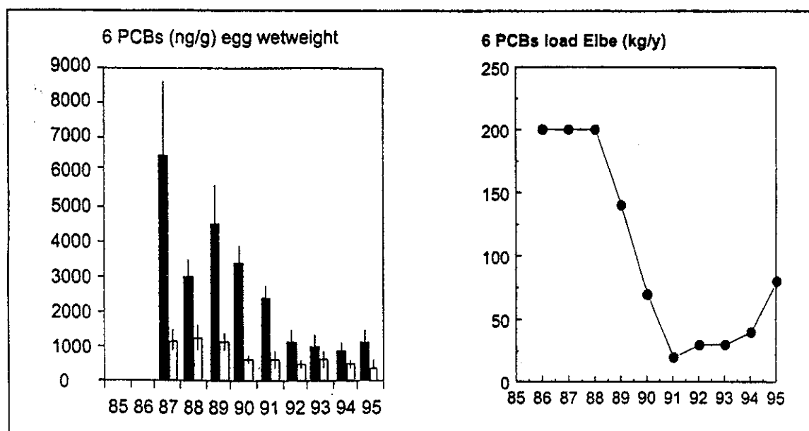
Figure A7.6. Temporal trend in PCB loads of the Elbe River compared to the trends in PCB concentrations in eggs of common terns (black columns) and oystercatchers (white columns) breeding at the Elbe estuary (Bakker et al. , 1997).
