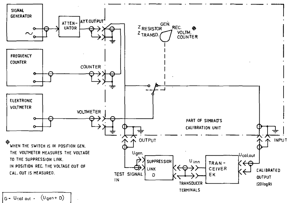
Figure 12b. Equipment set up for measuring the amplification (ref 3.4.3.3).
