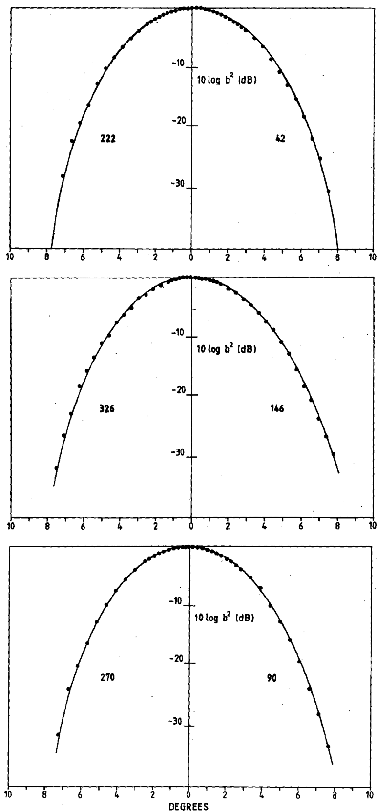
Figure 6. Measured two-way directivity patterns of the 38 kHz hull-mounted transducer on "Bjarni Saemundsson".
