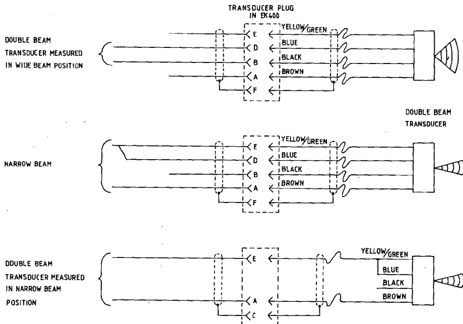
Figure 10b. Transducer connections for impedance measurement of the EK400 (ref 3.4.2.1).
