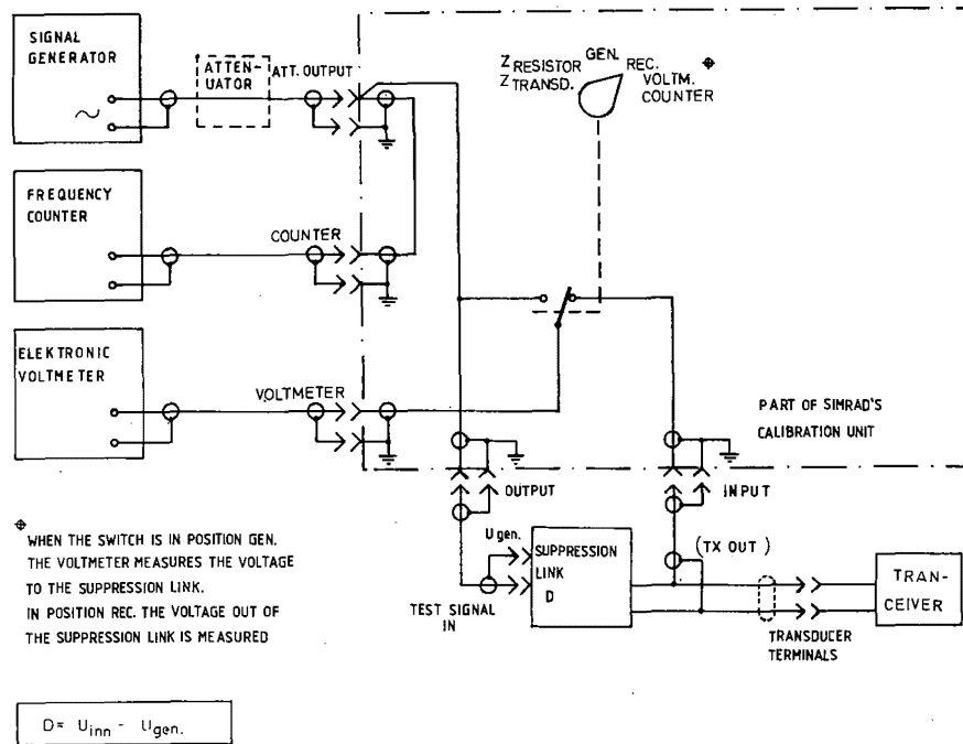
Figure 12a. Equipment set up for measuring the attenuator (ref 3.4.3.2).
