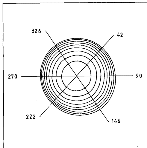
Figure 7. Equal-energy contours derived from the directivity patterns in Figure 6.
