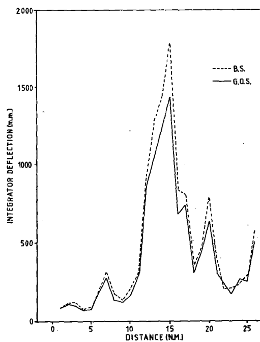
Figure 15. Illustration of echo abundance measures displayed for each mile sailed along a 26 mile course, obtained during the intercalibration of "Bjarni Saemundsson" and "G O Sars", October 1982.
