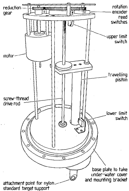
Figure 3. Mechanism for adjusting the length of twine supporting the standard target. Three such adjusters are shown at the arm ends in Figure 2.
