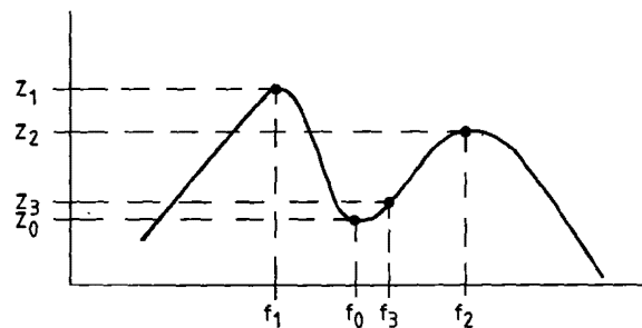
Figure 10c. Typical impedance characteristic.
