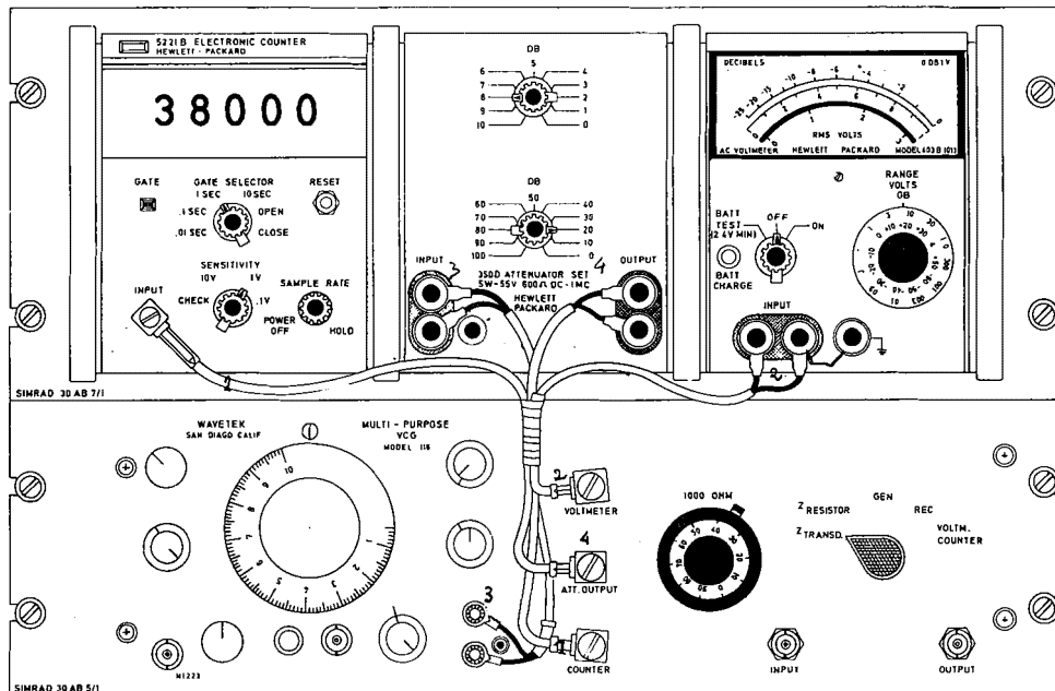
Figure 11b. Typical testing instruments.
