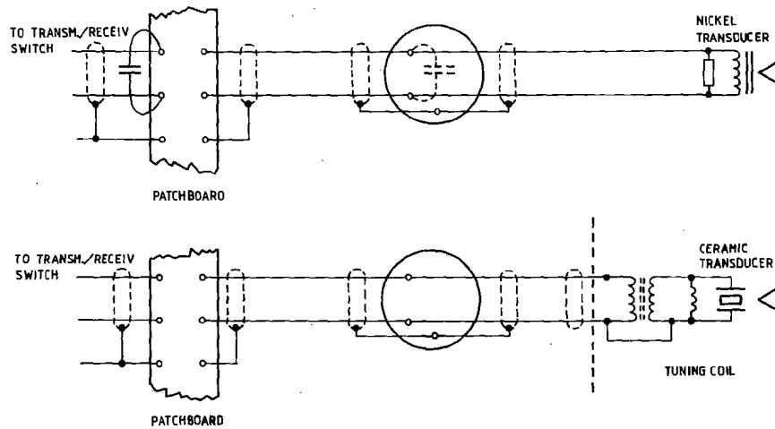
Figure 10a. Principal circuit diagram for nickel and ceramic transducers (ref 3.4.2).
