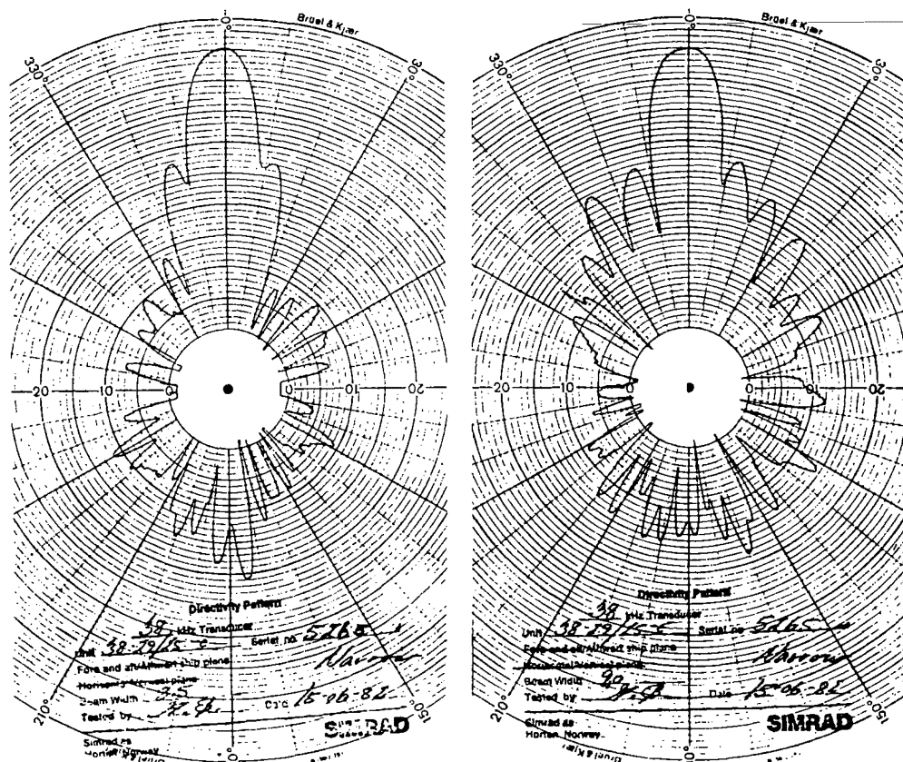
Figure 8. Laboratory measurements of the beam pattern of an unmounted transducer of the same model as that on "Bjarni Saemundsson".
