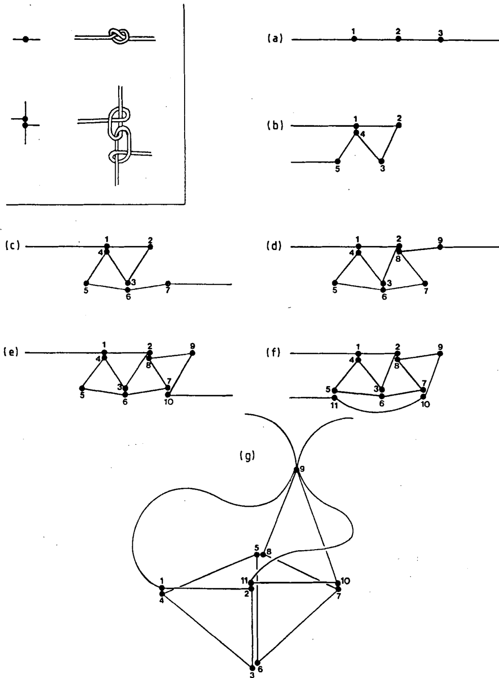
Figure 4. Construction of a monofilament container for standard target spheres. The numbers show the order of tying knots. Successive knots are one quarter of the sphere circumference apart.
