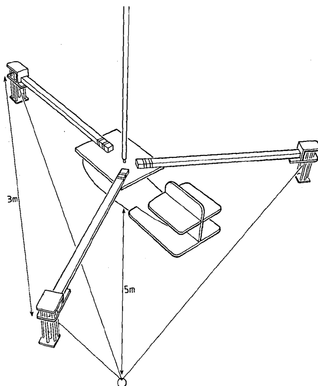
Figure 2. Rig and target suspension for towed-body calibration: moving sphere method.
