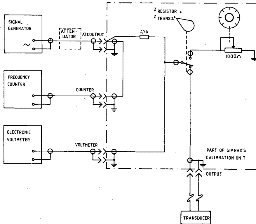
Figure 11a. Instrument configuration for impedance measurement.
