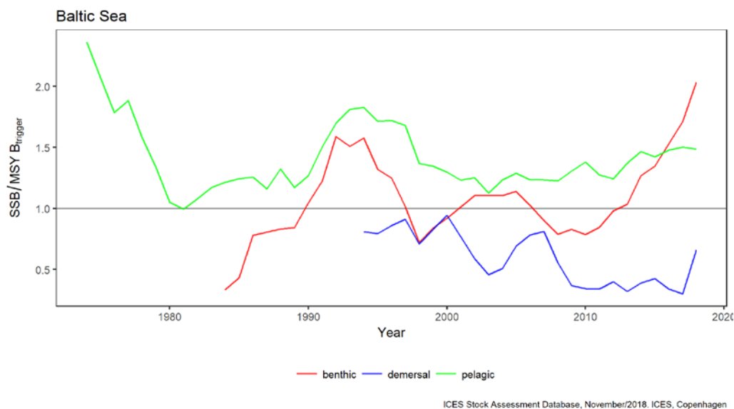
Figure 17 Time-series of average relative spawning-stock biomass (SSB to MSY B_{trigger} ratio) by fisheries guild for benthic, demersal and pelagic stocks (see Annex A).
