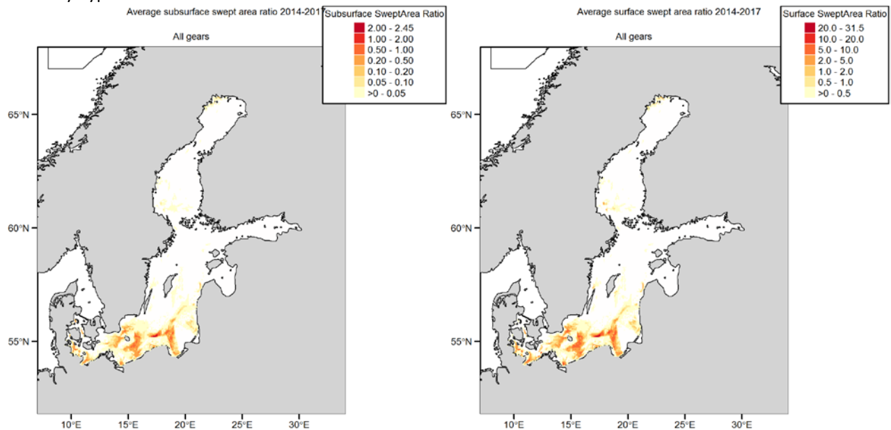
Figure 11 Average annual subsurface (left) and surface (right) disturbance by mobile bottom-contacting fishing gear (bottom otter trawls, bottom seines, beam trawls) in the Baltic Sea during 2014–2017, expressed as average swept area ratios (SAR).
