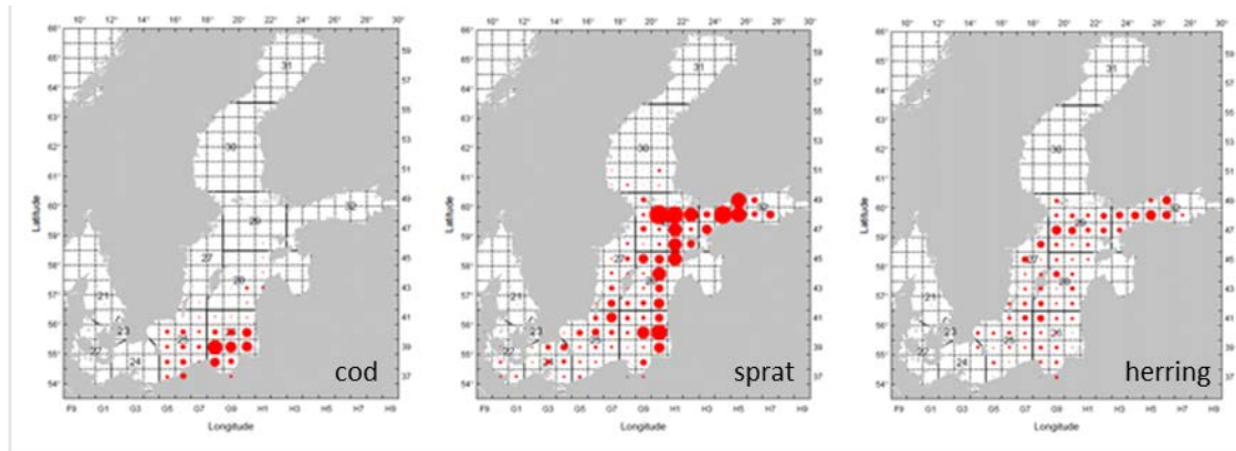
Figure 9** Left: Eastern Baltic cod \geq 30 cm in the Baltic international trawl survey (BITS, in numbers h^{-1} ) in the 4th quarter 2017. Middle: Sprat (ages between 1 and 8) in the Baltic international acoustic survey (BIAS, in numbers) in the 4th quarter 2017. Right: Herring in subdivisions 25–29 and 32, excluding the Gulf of Riga, from the BIAS survey (BIAS, in numbers) in the 4th quarter 2017. Note that all figures are based on number of individuals and not on biomass. The BIAS survey does not cover the Gulf of Bothnia or the Bothnian Sea.
