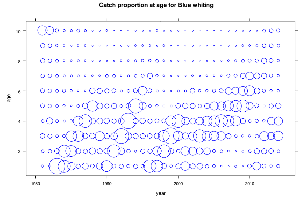
Figure D3. Catch numbers-at-age mean standardised by year 1981–2014.
