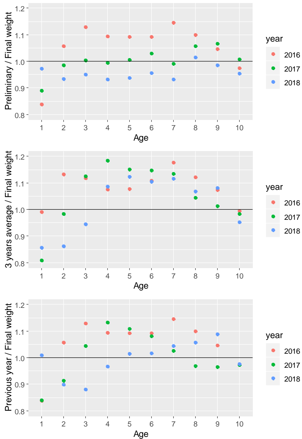
Figure B3. Comparison of preliminary mean weight at age for potential use in the assessment and final mean weight. The upper panel compares the preliminary weights with the final weights (obtained in the following year). The middle panel shows the average of the 3 preceding years weights compared with the final weights. Bottom panel shows previous years weights compared with the final year.
