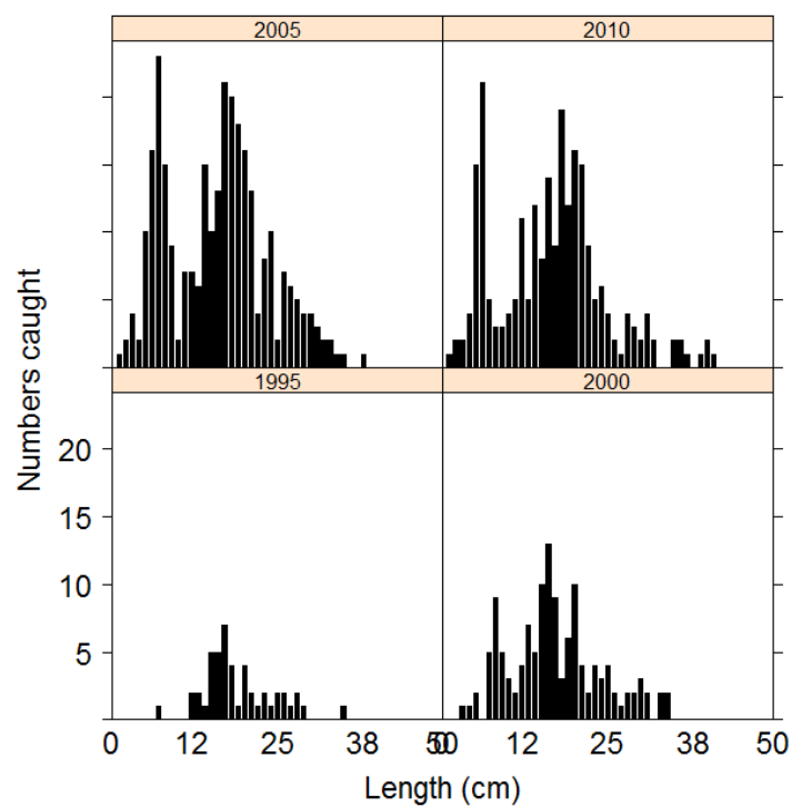
Figure 2.17. Length distributions of brill Scophthalmus rhombus caught by BITS_HAF_Q1&4 in the Kattegat (3.aS).
