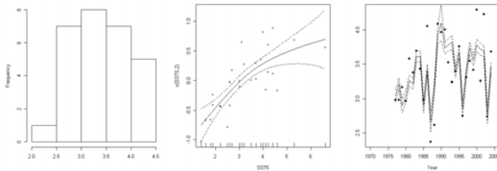
b) Diagnostic plots of the finally selected environment-recruitment models using Rs (hier model); from left to right: distribution of residuals, effect of SST in May (SST5), predicted (lines with 95% confidence limits) vs. observed (points) Rs.
