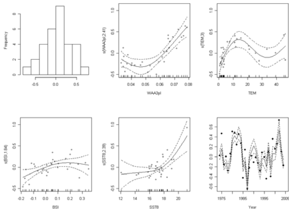
a) Diagnostic plots of the finally selected environment-recruitment models using Ra (hier model); from left to right: distribution of residuals, effect of individual weight (WAA3pl – mean weight of age-groups 3+), effect of T. longicornis biomass (TEM), effect of the Baltic Sea indec (BSI), effect of SST in August (SST8), predicted (lines with 95% confidence limits) vs. observed (points) Ra.
