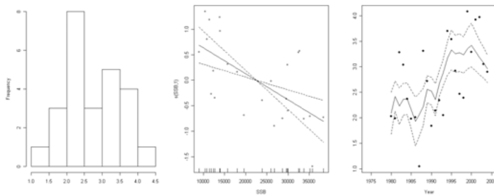
a) Diagnostic plots of the finally selected environment-recruitment models using R_s (hier model); from left to right: distribution of residuals, effect of spawning stock biomass (SSB), predicted (lines with 95% confidence limits) vs. observed (points) R_s .
