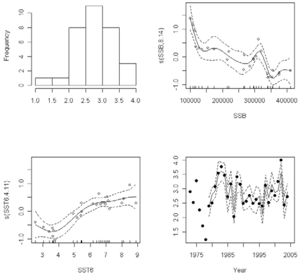
b) Diagnostic plots of the finally selected environment-recruitment models using R_s (hier model); from left to right: distribution of residuals, effect of spawning stock biomass (SSB), effect of SST in June (SST6), predicted (lines with 95% confidence limits) vs. observed (points) R_s .
