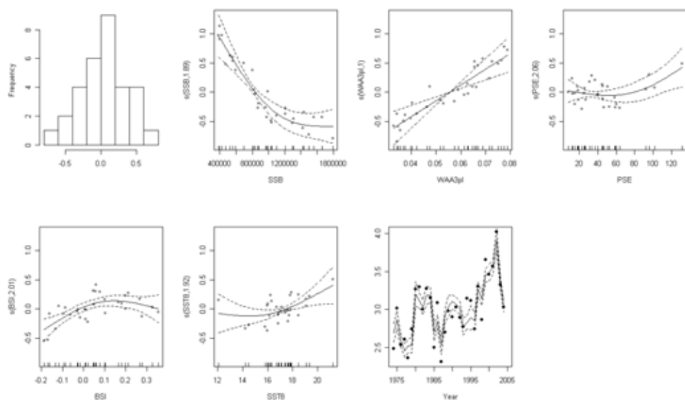
b) Diagnostic plots of the finally selected environment-recruitment models using Rs (hier model); from left to right: distribution of residuals, effect of spawning stock biomass (SSB), effect of individual weight (WAA3pl – mean weight of age-groups 3+), effect of P. acuspes biomass (PSE), effect of the Baltic Sea indec (BSI), effect of SST in August (SST8), predicted (lines with 95% confidence limits) vs. observed (points) Rs.
