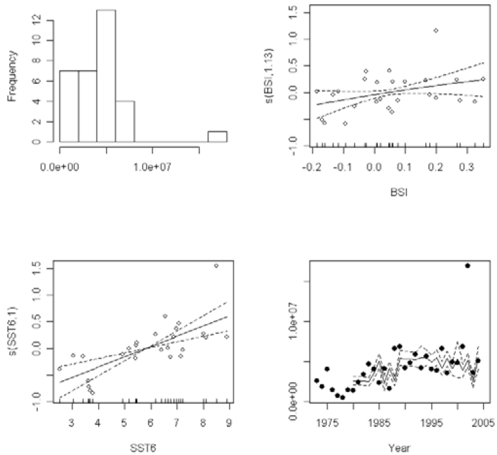
a) Diagnostic plots of the finally selected environment-recruitment models using R (hier model); from left to right: distribution of residuals, effect of the Baltic Sea Index (BSI), effect of effect of SST in June (SST6), predicted (lines with 95% confidence limits) vs. observed (points) R.
