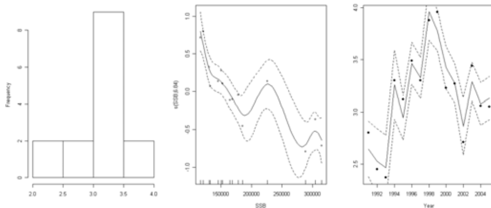
b) Diagnostic plots of the finally selected environment-recruitment models using Rs (hier model); from left to right: distribution of residuals, effect of spawning stock biomass (SSB), predicted (lines with 95% confidence limits) vs. observed (points) Rs.
