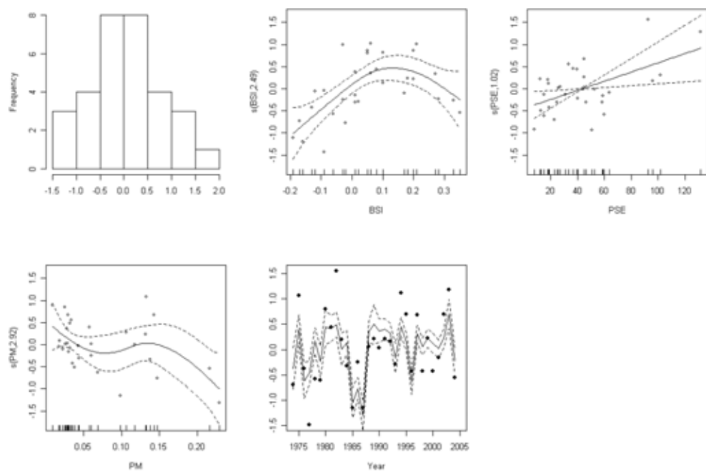
a) Diagnostic plots of the finally selected environment-recruitment models using R_a (hier model); from left to right: distribution of residuals, effect of the Baltic Sea Index (BSI), effect of P. acuspes biomass (PSE), effect of cod predation (PM), predicted (lines with 95% confidence limits) vs. observed (points) R_a .
