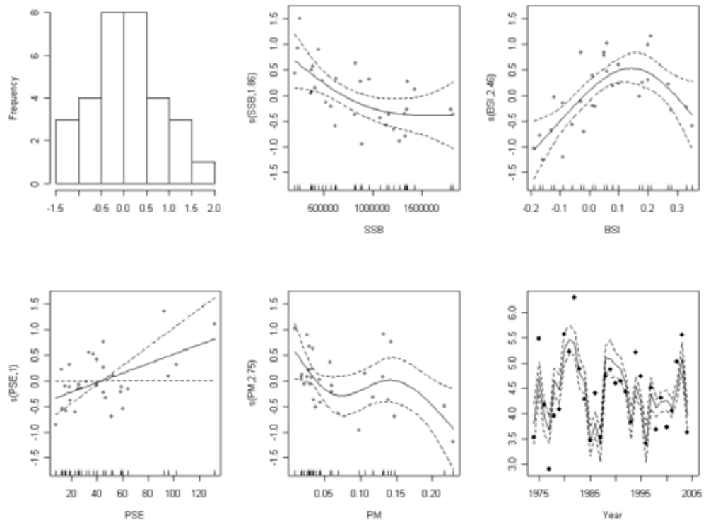
b) Diagnostic plots of the finally selected environment-recruitment models using R_s (hier model); from left to right: distribution of residuals, effect of spawning stock biomass (SSB), effect of the Baltic Sea Index (BSI), effect of P. acuspes biomass (PSE), effect of cod predation (PM), predicted (lines with 95% confidence limits) vs. observed (points) R_s .
