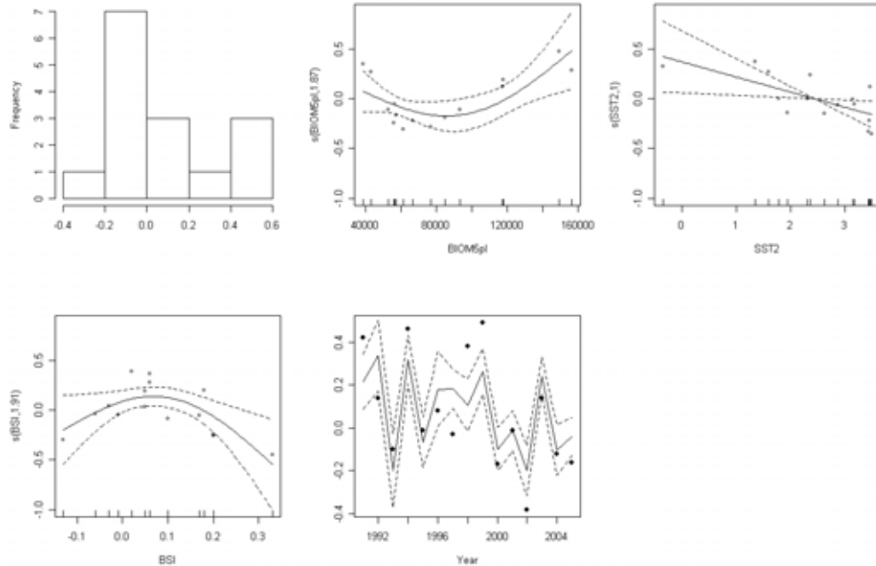
a) Diagnostic plots of the finally selected environment-recruitment models using Ra (hier model); from left to right: distribution of residuals, parental effect of older individuals (BIOM5pl – biomass of age-groups 5+), effect of surface salinity in February (SST2), effect of the Baltic Sea index (BSI), predicted (lines with 95% confidence limits) vs. observed (points) Ra.
