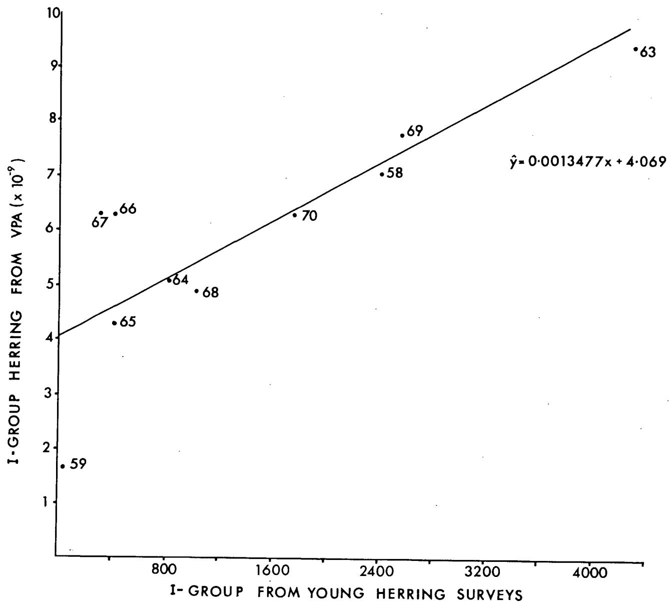
Figure 9. Calculated regression line of year class strength estimates obtained from VPA and International Young Herring Surveys.
