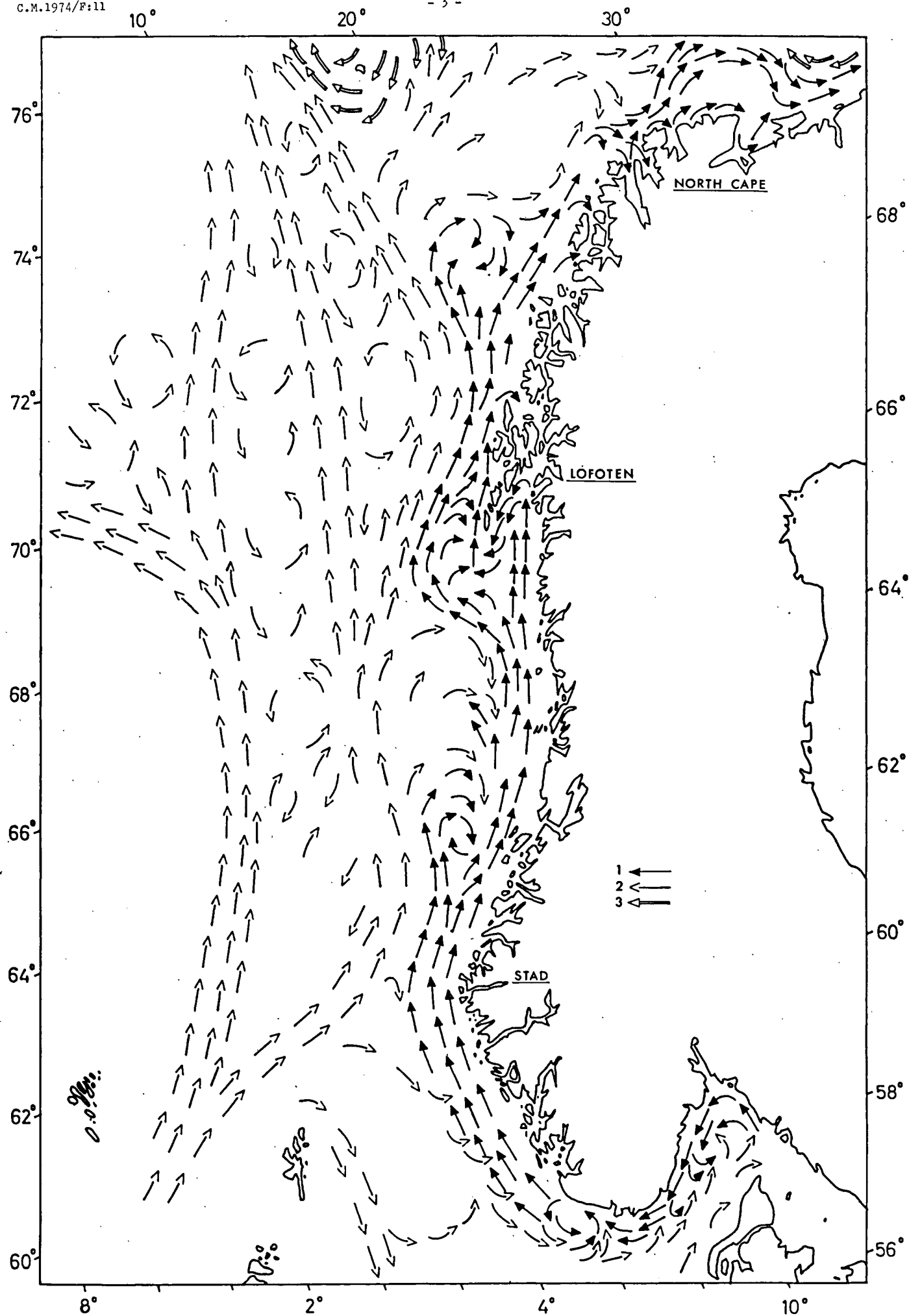
FIGURE 1. DISTRIBUTION OF WATER MASSES AND CURRENTS OFF THE NORWEGIAN COAST, 1) COASTAL WATER, 2) ATLANTIC WATER, 3) POLAR WATER (FROM SETRE AND LJOEN 1972).
