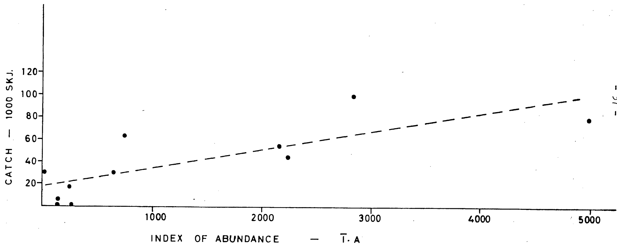
Figure 12. Comparison between 0-group sprat abundance and subsequent catch.
