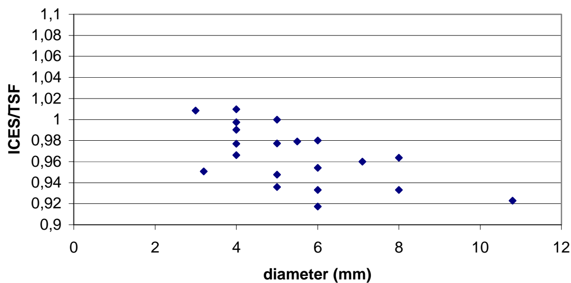
Figure 2. Ratio ICES/TSF in relation to twine diameter for all mesh constructions.
