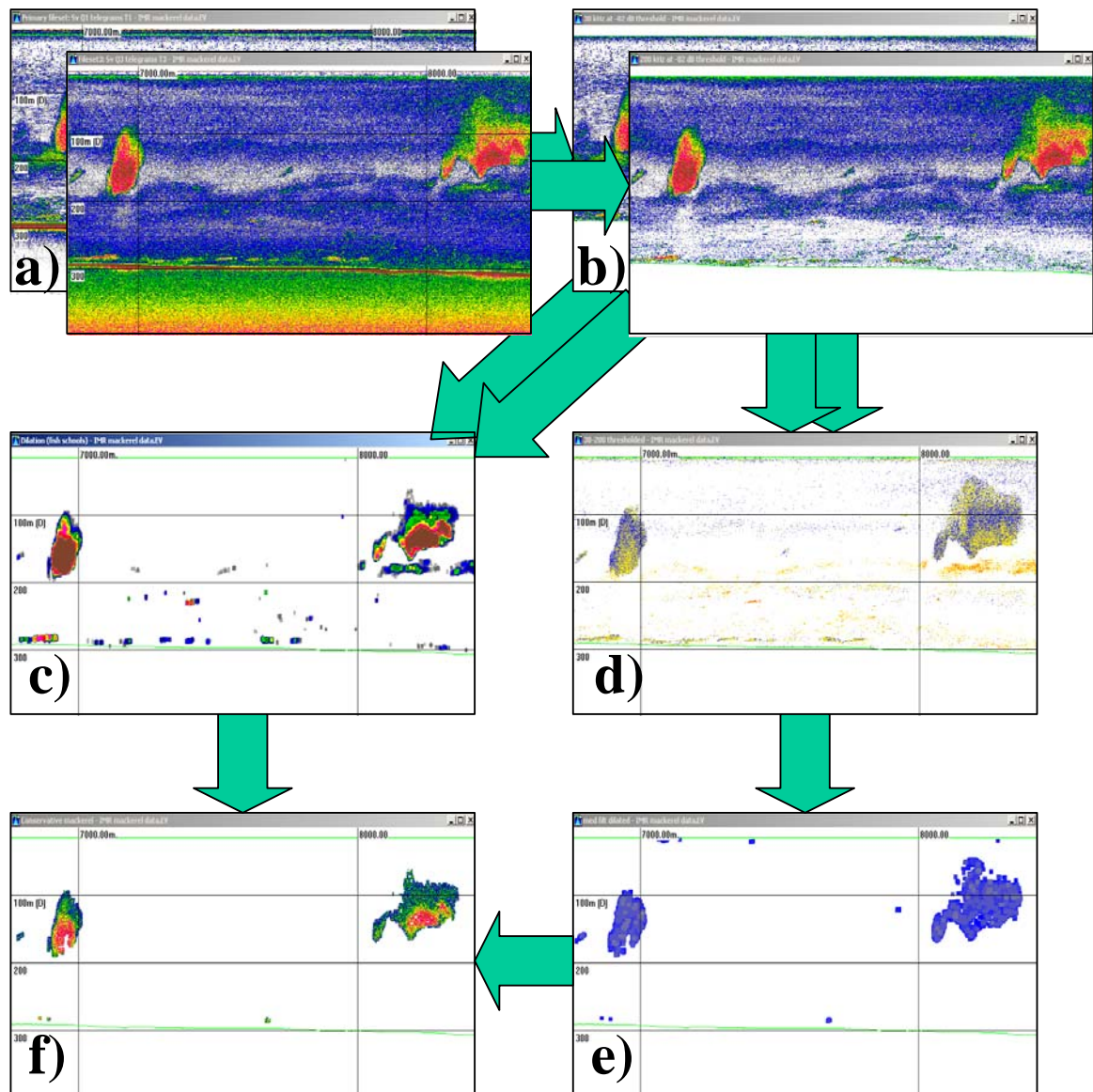
Figure 3.3.2. Six major processing steps in the FRS mackerel algorithm; the virtual echogram names are given in italics . a) Raw data (MVBS) at 38, 120 (not shown) and 200 kHz. b) 38 and 200 kHz MVBS filtered for noise, seabed and transmit pulse, 38 kHz at -82 dB threshold & 200 kHz at -82 dB threshold; the processed data are input to both of the following processes. c) potential fish school after non-fish filtration, Dilation (fish schools); d) 38-200 dB difference echogram, 38-200 thresholded; e) potential mackerel schools echogram, med filt dilated; f) final output, conservative mackerel echogram.
