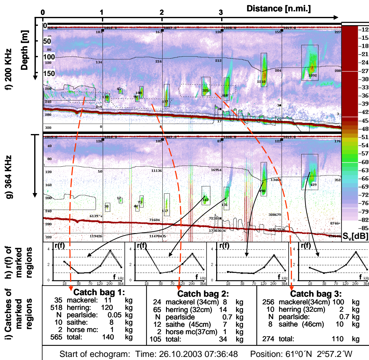
Figure 3.2.7 (f-i). The 200 kHz and 364 kHz data are shown at the top. In the 200 kHz echogram, the three polygons mark each of the three bags of the opening-close trawl system. The catches are shown in Figure i. The vertical dark-red lines in the middle of Figure g is due to noise.
