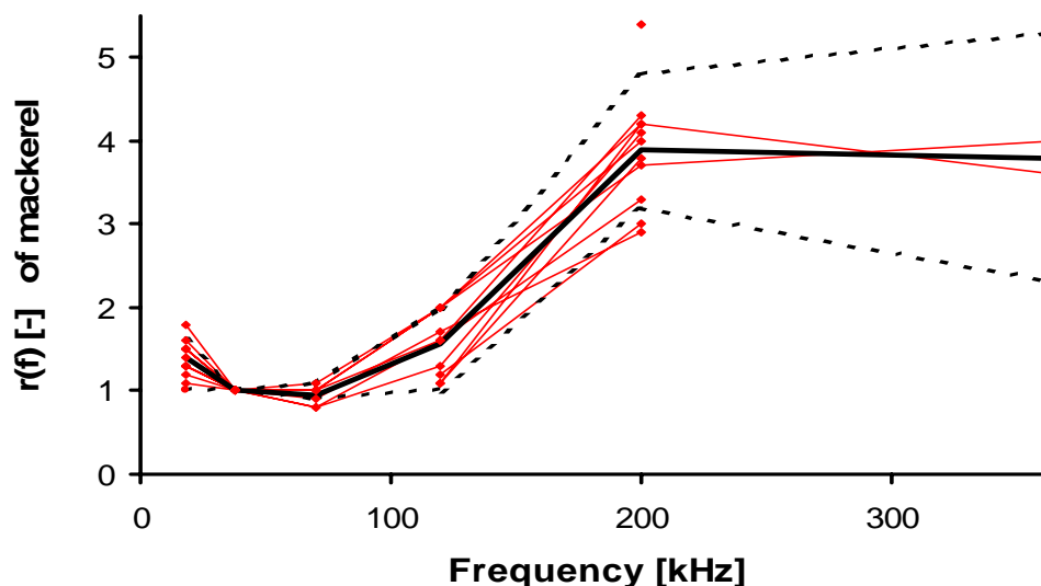
Figure 3.2.5: Measured relative frequency response, r(f) for mackerel. Red curves are average either per cruise or per cage measurement series.
