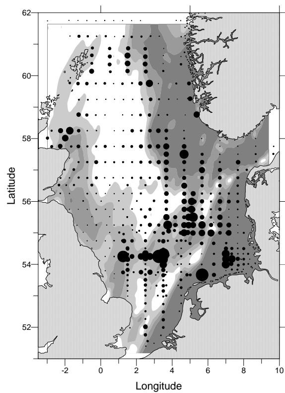
Figure 10-6: Relative abundance of cod eggs against rate of change in sigma-t (area of circles indicates \text{no m}^{-2} ).
