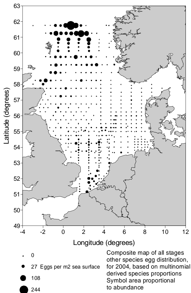
Figure 7-4: OTHER SPECIES WITH COD-LIKE EGGS (eggs of diameter 1.1 – 1.75 mm and lacking oil globules or other distinguishing features) - distribution (all developmental stages) in 2004.
