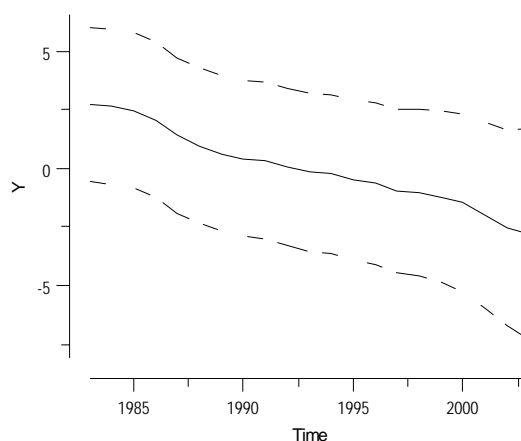
Figure 4–2: Common trend in herring, sandeel and Norway pout standardized recruitments series (1983–2003) and 95% confidence interval of the DFA model (AIC = 187.47).
