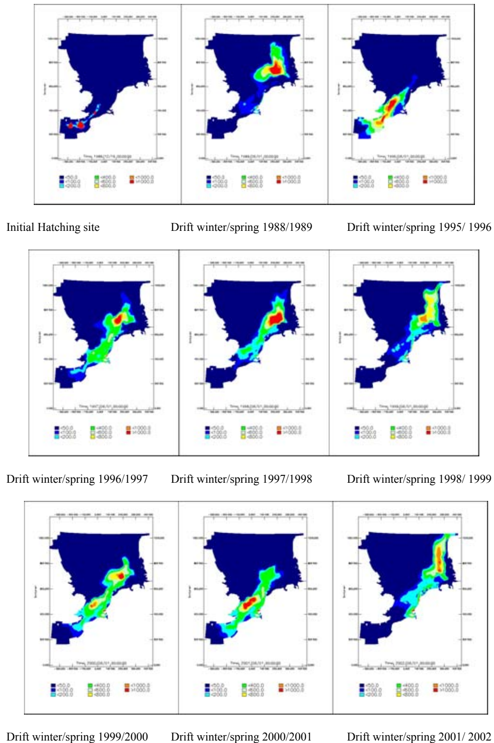
Figure 3.1.4: North Sea Herring – Predicted concentrations of late stage postlarvae in late May by year: Results of transport simulations of herring larvae using the WL model (Delft Hydraulics) from hatch to the end of May for 8 selected years. Larvae given diel behaviour as the develop. See Bolle et al (2005) for full details
