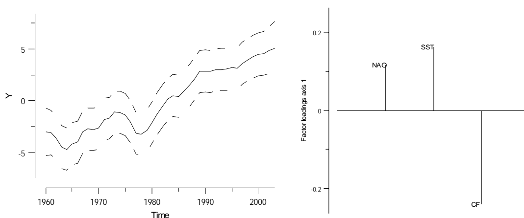
Figure 5.1.2: Trend in time-series of North Atlantic Oscillation Index (NAO), annual mean North Sea surface temperature (SST) and the annual mean abundance of Calanus finmarchicus (from CPR data). Dynamic factor analysis (see section 4 for methods) revealing increasing trend in NAO and SST and declining trend in C. finmarchicus abundance. Note there is no relationship between NAO and SST for the shorter time-series (1983–2003).
