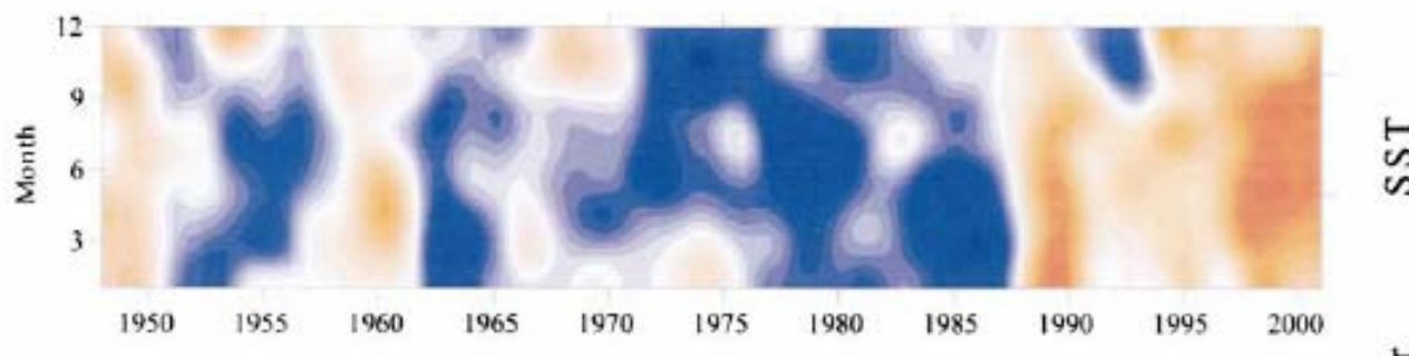
Figure 5.1.1: Monthly standardized anomaly plots for sea surface temperature (1948–2002). Shades of red signify values above the long-term mean and shades of blue values below the long-term mean. Zero-mean values are in white. Data averaged for the central North Sea. From Edwards, M., D. G. Johns, S. C. Leterme, E. Svendsen, and A. J. Richardson. 2006. Regional climate change and harmful algal blooms in the Northeast Atlantic. Limnol. Oceanogr. 51: 820–829
