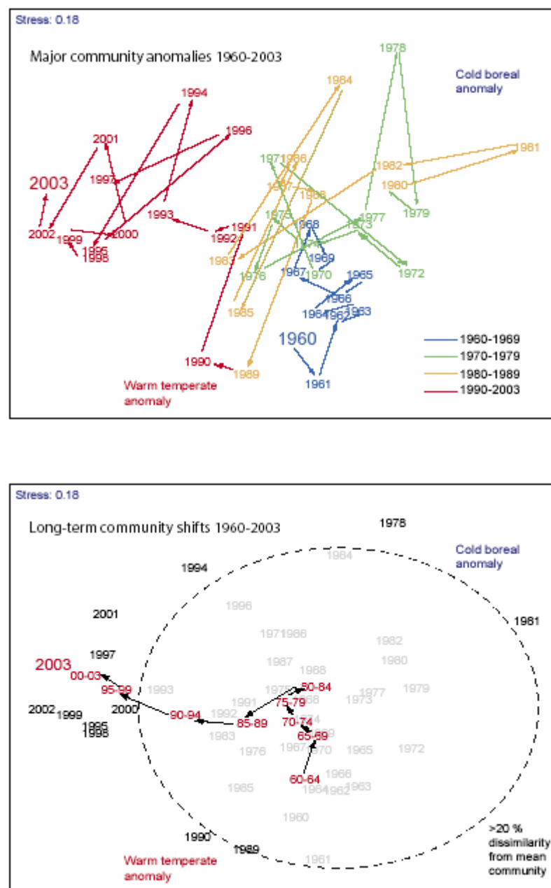
Figure 5.2.1: Multi-dimensional scaling plot of the annual zooplankton community structure in the central North Sea from 1960–2003 revealing major structural shifts (top figure) and five-year community averages (bottom figure). Similarity matrix based on Bray-Curtis and \log(x+1) transformations (Edwards et al., 2005).
