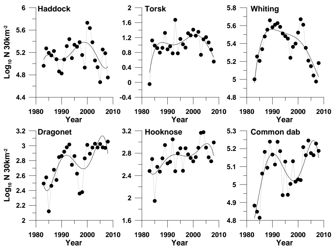
Figure 3.6. Trends in the standardised \log_{10} abundance of the three species, haddock, torsk, and whiting, positively related to Factor 2 and the three species, dragonet, hooknose (pogge), and common dab, positively related to Factor 7. Abundance data are derived from the Q1 IBTS. Smoothers are 5 th degree polynomials.
