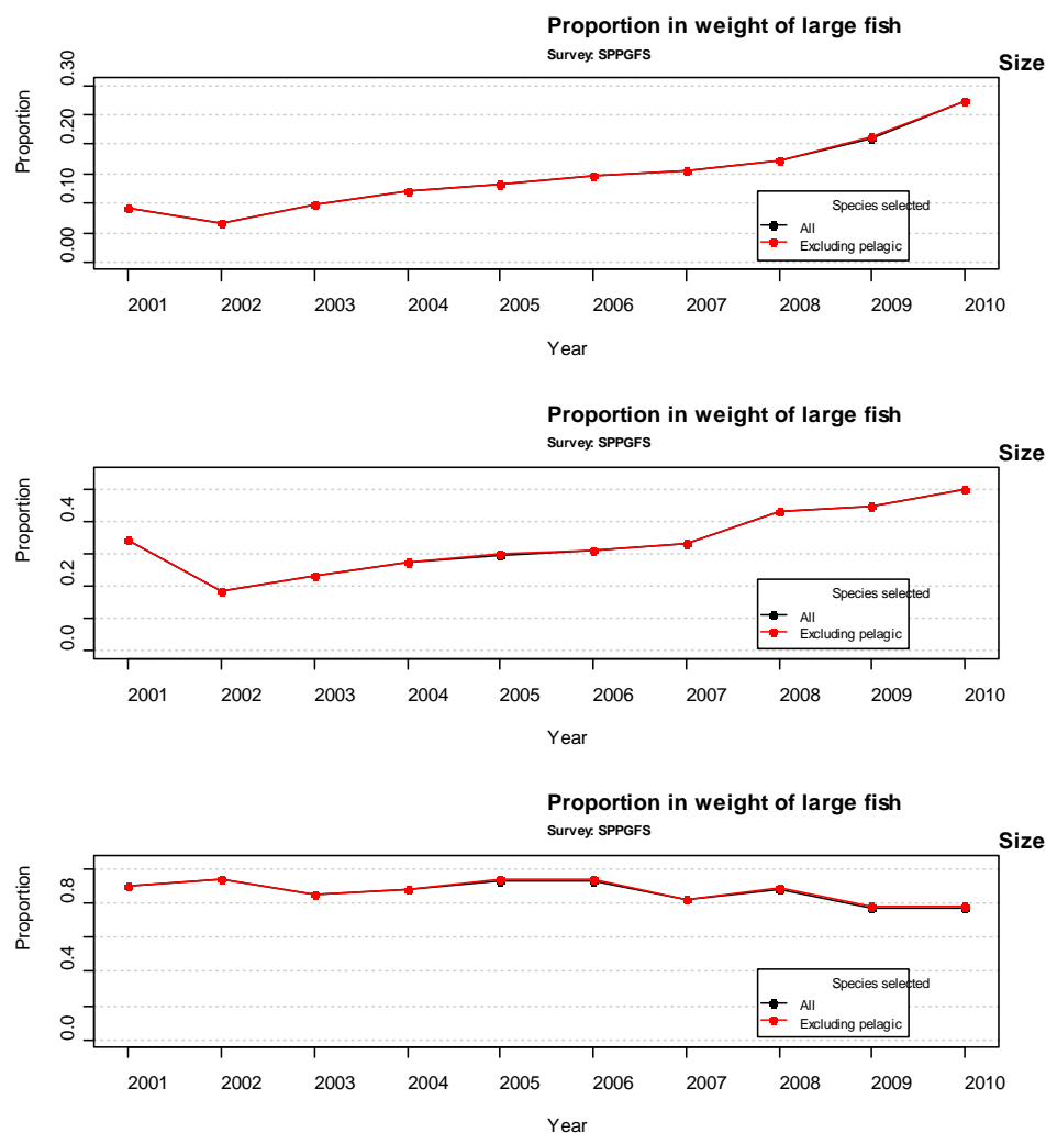
Figure 5.2. LFI variation using three different length thresholds (top to bottom: 40 cm, 30 cm, 20 cm) to define large fish, and including pelagic fish (black line) and excluding pelagic fish (red line). Data from the Spanish Porcupine Bank survey (2001–2010).
