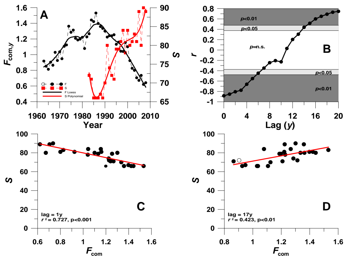
Figure 3.3. A: Trends in North Sea demersal fish species richness (S) and an indicator of community averaged fishing mortality (F com ). Loess smooths are fitted to the two trend lines. B: variation in the correlation between the two trends at various lags, where the lag represents the period in years (y) separating the date of the species richness observation and the number of years previously that fishing mortality indicator was determined. Negative correlations are shown for illustrative purposes, indicating when the relationship between the two metrics was negative. C: and D: examples of the relationship between species richness and fishing mortality at lags of 1y and 17y respectively. Certainly marked changes in the abundance of nominally ‘rare’ species have been documented, and these have influenced whether or not these species are detected in the IBTS or not (Harris et al. , 2007).
