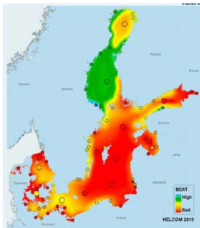
Figure 2.1. Preliminary integrated classification of biodiversity status of the Baltic Sea. Explanation on the methodology behind the status assessment is found in HELCOM (2009). There is a gradient ranging from unacceptable (warm colours) to acceptable biodiversity status. The circles represent the assessment sites.
