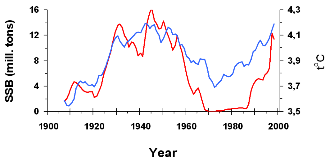
Figure 17. Spawning stock biomass of Norwegian spring-spawning herring and the long-term-averaged sea surface temperature or AMO (Toreisen and Østvedt, 2000).
