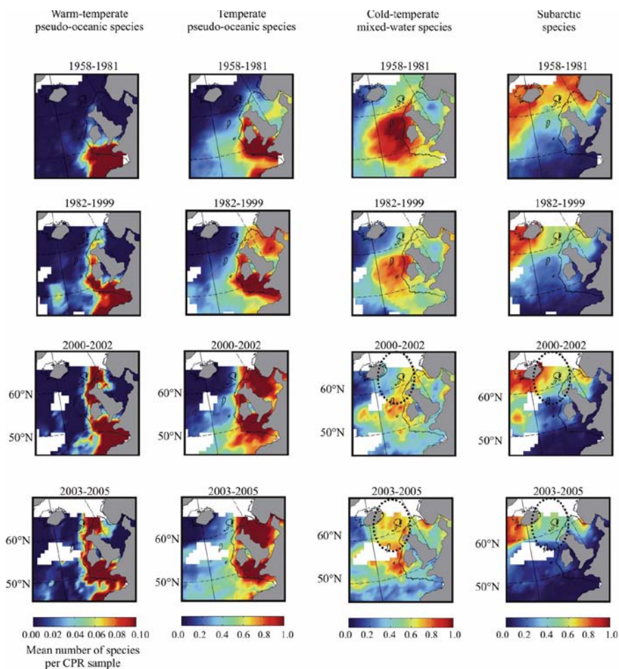
Figure 21. Biogeographical changes in four plankton assemblages spanning five decades. Warm water plankton are moving north and cold water plankton are moving out of the North Sea.
