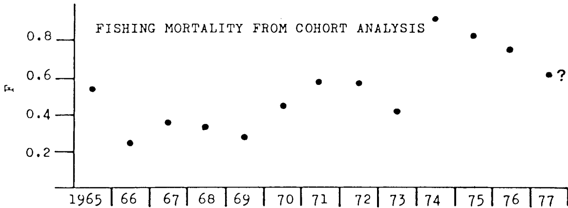
APPENDIX Figure 2. IRISH SEA HERRING. Division VIIa. Exploited Manx stock. Biomass, catch, effort and fishing mortality, 1965-77.
