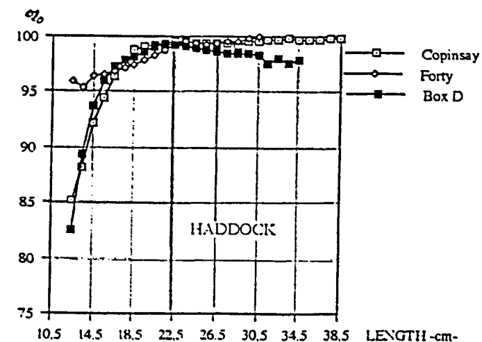
Fig. 7.4.2 CATCHING EFFICIENCY OF MAIN TRAWL AT DIFFERENT FISHING PLACES
