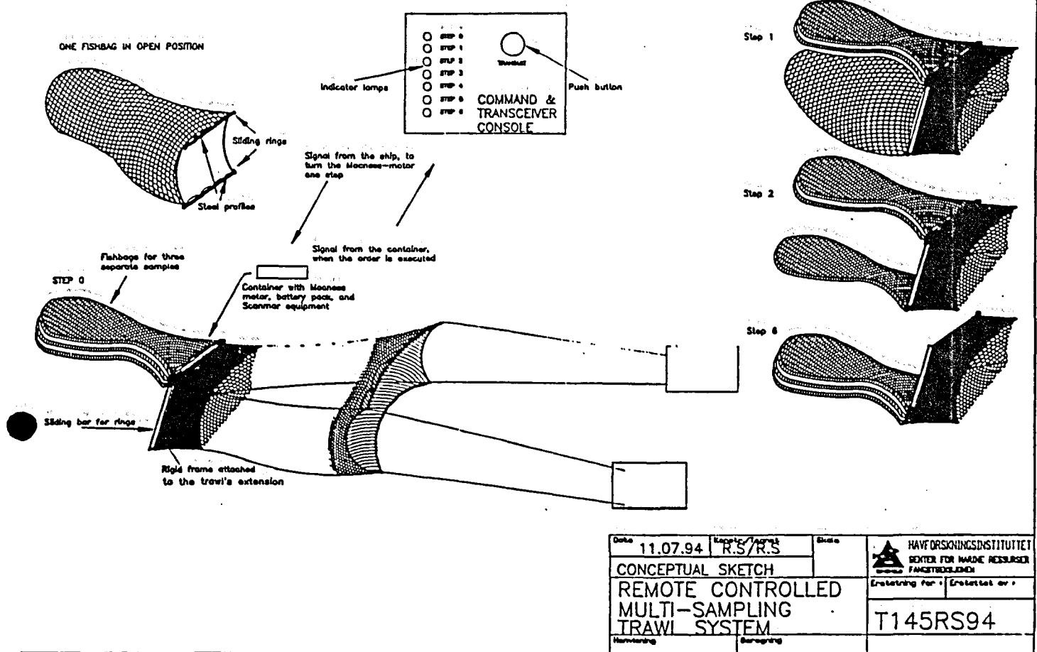
Fig. 7.1.1 Multi-Sampler: a remote controlled multi-sampling trawl system
