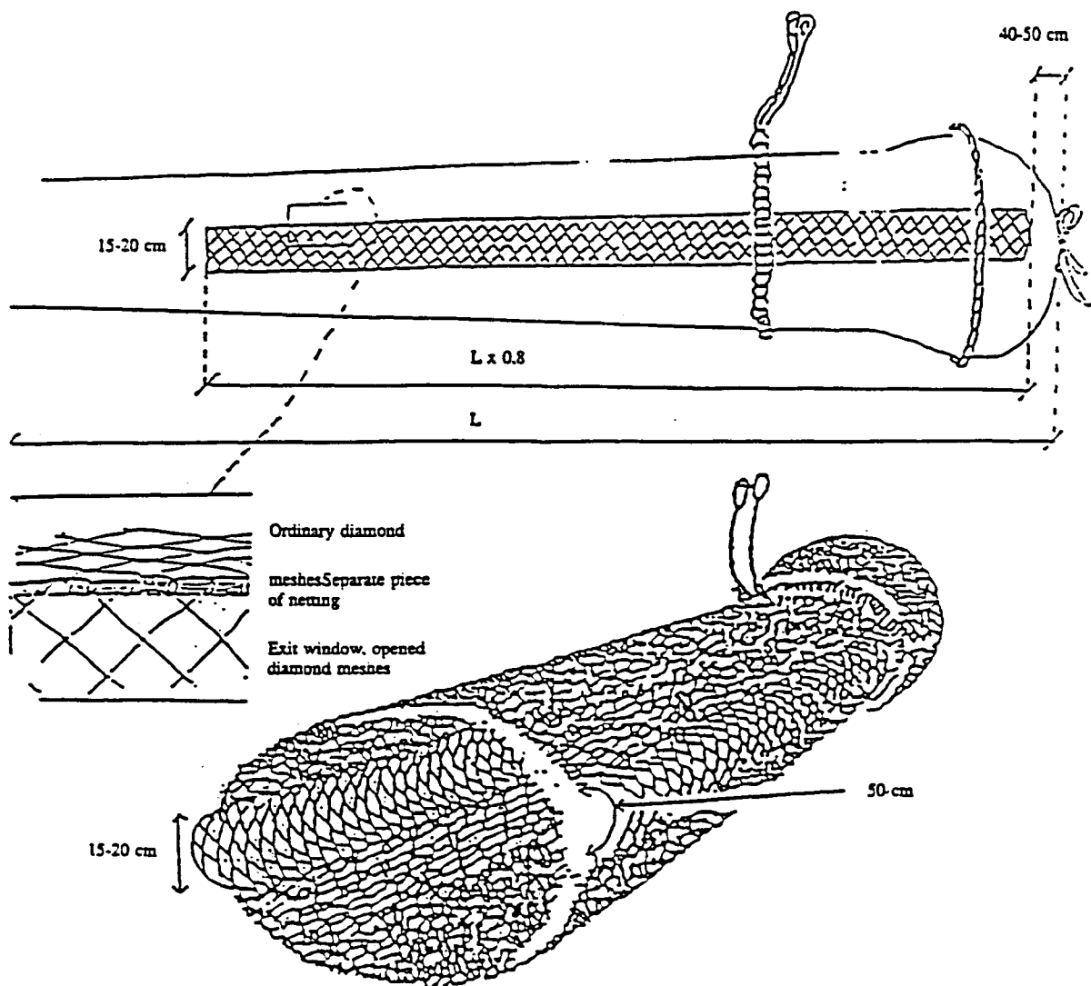
Diagram (Exit window model 1)
