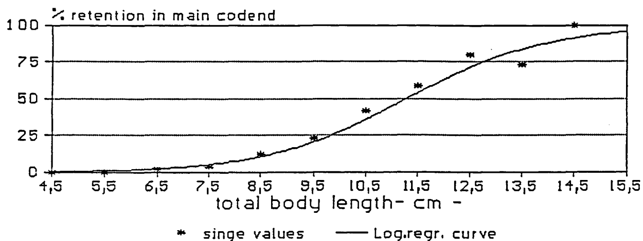
Fig. 7.3.1 Catching efficiency of codhopper for Nephrops norvegicus Selection by the roller gear
