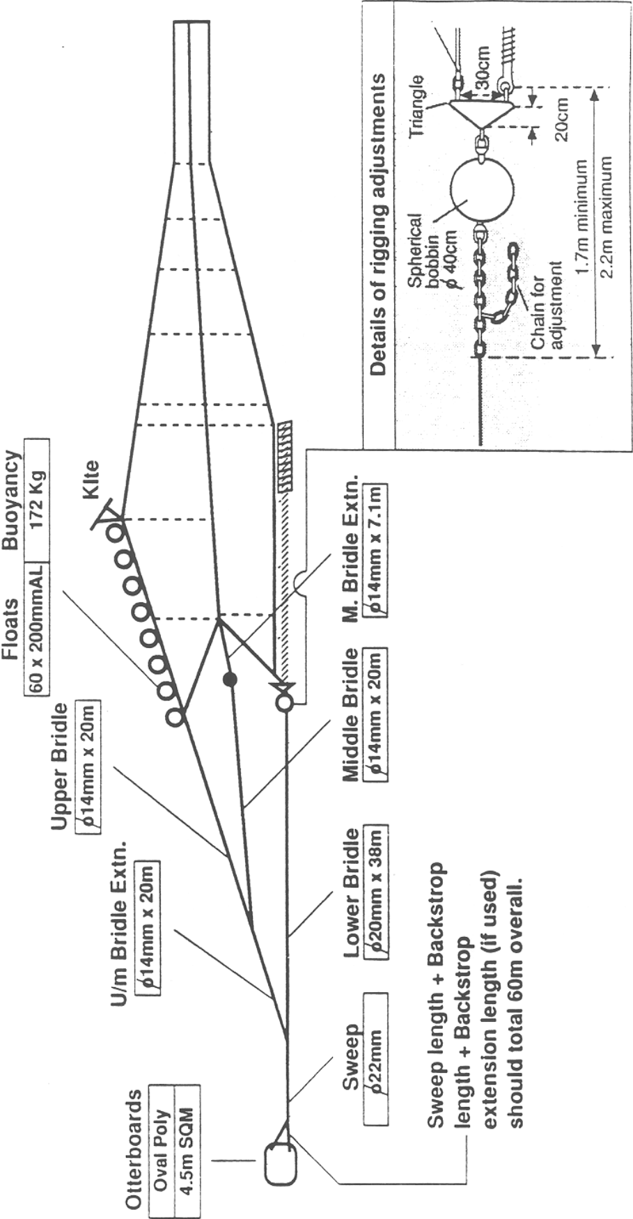
Figure 2.5 Rigging of the 36/47 GOV Trawl
