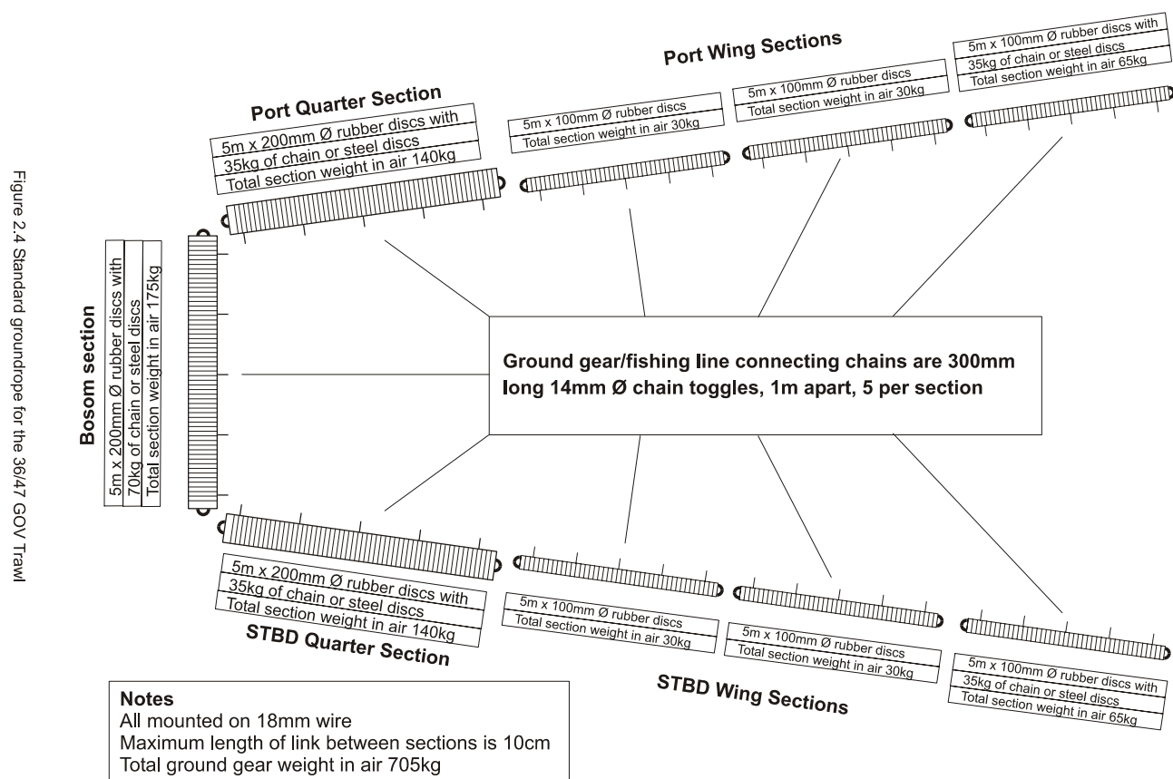
Figure 2.6 Standard groundrope for the 36/47 GOV trawl ground gear 'A'
