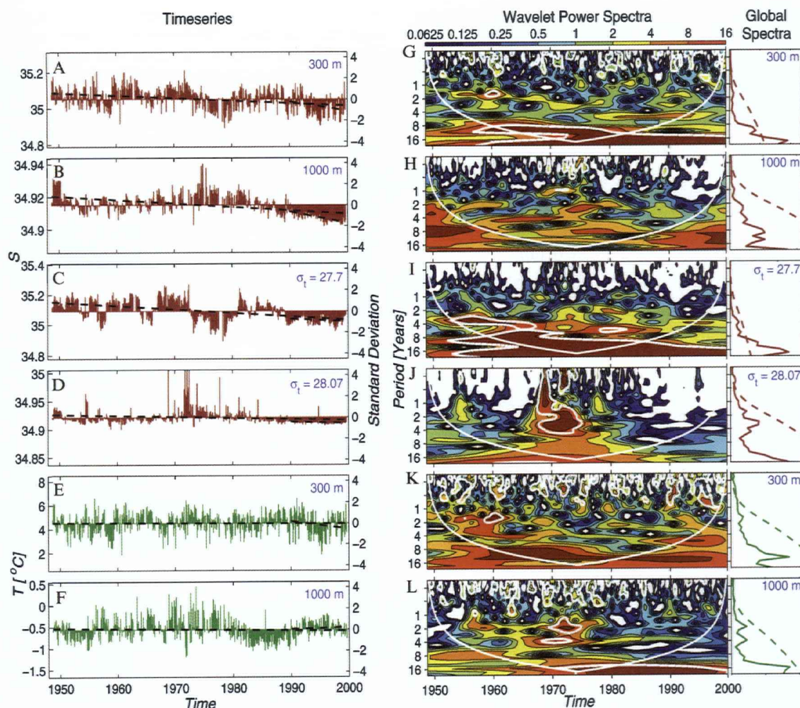
Figure 3. Time-series of monthly salinity at two chosen standard depths (A, B) and at their corresponding isopycnal surfaces (C, D), and time-series of monthly temperature at same depths (E, F). Since salinity and temperature are closely allied on the same isopycnal surface, isopycnal series of temperature is also represented by (C, D). Dashed lines represent linear trends. Panels G-L show Wavelet Power Spectra of variance normalized by 1/\sigma^2 . White curves give "Cones-of-Influence" outside which edge effects affect the result. White contours enclose regions of greater than 95% confidence for a red noise process with a lag1 coefficient of 0.72. The global wavelet spectrum is similar to a "regular" (Fourier) spectrum for the whole time-series, and here plotted together with the mean red noise spectrum (dashed line).
