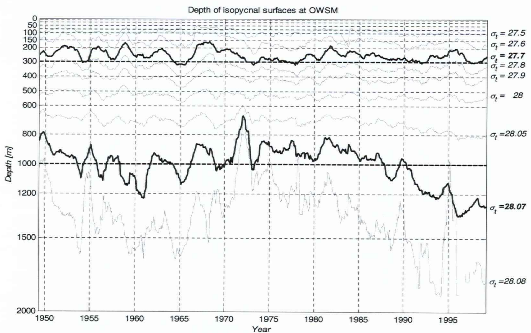
Figure 2. Time-series of the depth of chosen isopycnal surfaces, smoothed by a simple 1-year wide boxcar filter. The thick lines represent the depths and isopycnal levels analysed in Figure 3.
