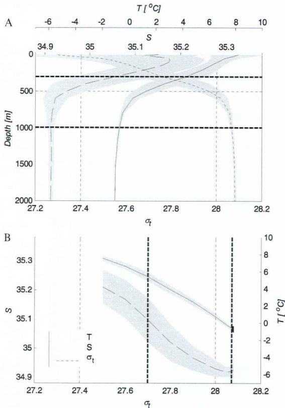
Figure 1. Average profiles from OWSM in depth (A) and sigma coordinates (B). Shaded regions illustrate standard deviation. As can be seen, these are in the pycnocline and the intermediate/deep waters, respectively.
