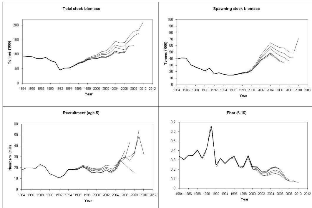
Figure 21.1 Retrospective analysis
