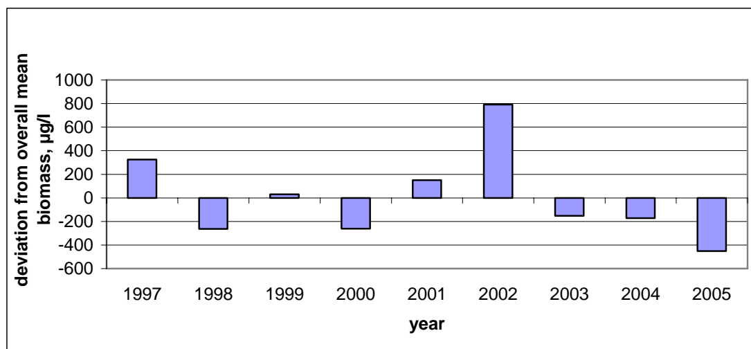
Figure 12.5.1: Relative biomass of N 2 -fixing cyanobacteria (µg/l) along a cross-section of the central Gulf of Finland, Baltic Sea. The overall mean is calculated as an average of all observations during the period from 15 June to 31 July in 1997–2005.
