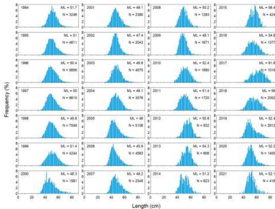
Figure 5.6.5. Length distributions of the catch of tusk by Faroese longliners (>100 BRT) in Division 5.b. ML- mean length in cm, N- number of length measures.
