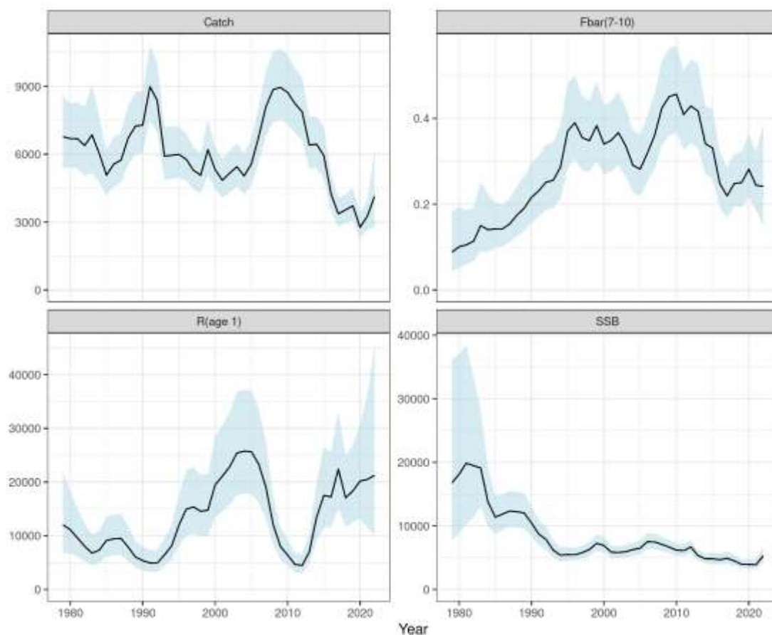
Figure 5.2.16: Tusk in 5.a and 14. Model results of population dynamics overview: estimated catch, average fishing mortality over ages 7 - 10 ( F_{bar} ), recruitment (age 1), and spawning stock biomass (SSB).
