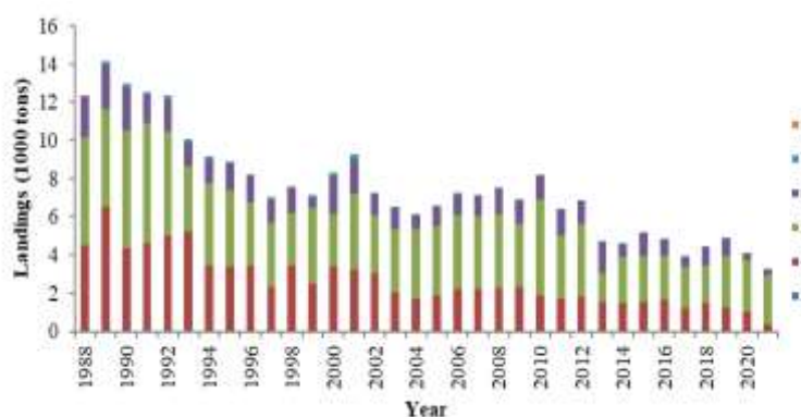
Figure 5.6.1. Landings of tusk per year for 1988–2021.
