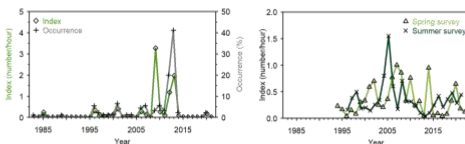
Figure 5.6.10. Tusk 5.b. Abundance index for tusk (2–3 cm in length in number/hour) on the Faroe Plateau based on the 0-group survey (left figure) and abundance index for tusk < 40 cm from the annual spring and summer trawl survey on the Faroe Plateau (right figure).
