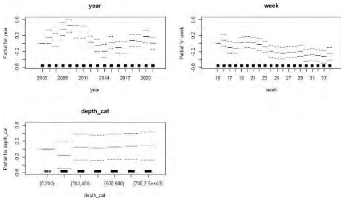
Figure 6: ARU.27.5b6a standardized CPUE explanatory variables
