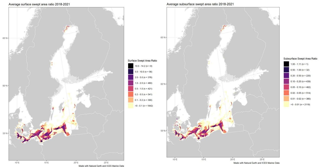
Figure 11 Average annual surface (left) and subsurface (right) disturbance by mobile bottom-contacting fishing gear (bottom otter trawls, bottom seines, beam trawls) in the Baltic Sea during 2018–2021 (with available data), expressed as average swept area ratios (SAR).
