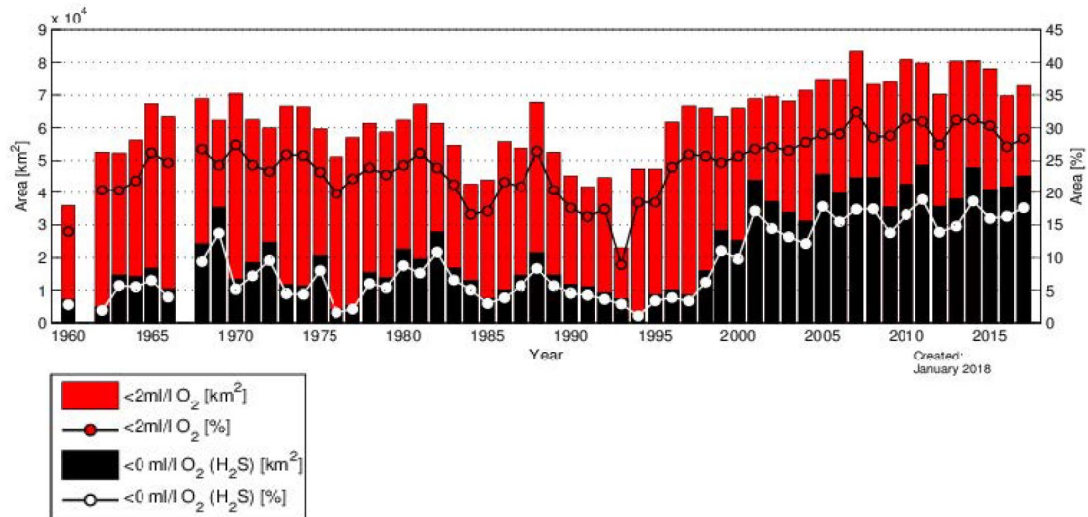
Figure 14 Extent of hypoxic and anoxic bottom water in the central Baltic and Gulf of Finland, 1960–2017.
