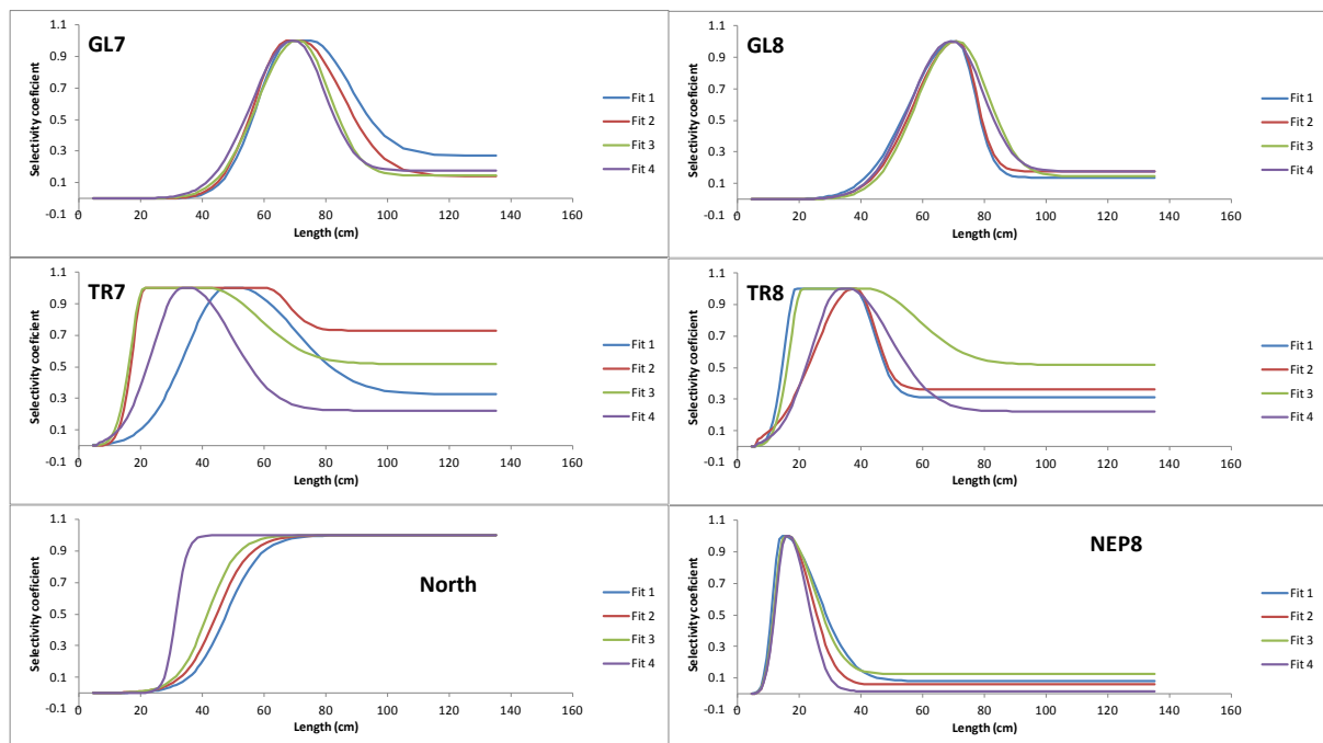
Figure 4. Estimated northern hake selectivity coefficients by commercial fleets for the 4 fits (see text for fit settings).
