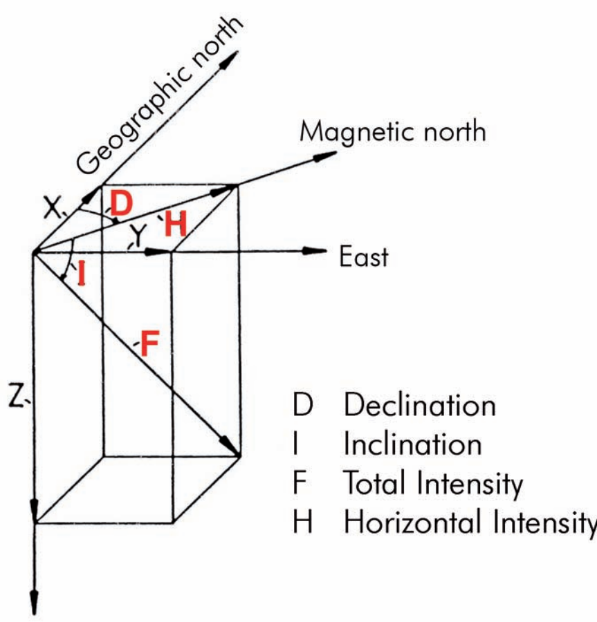
Figure 2: elements of the earth’s magnetic field vector.
