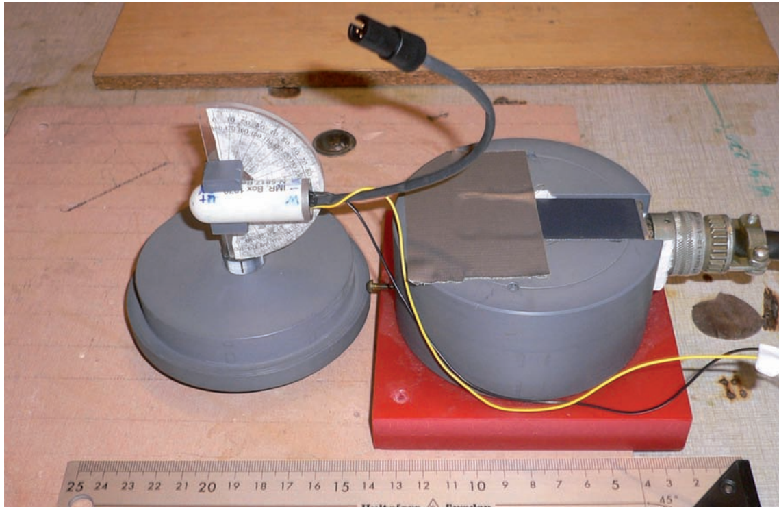
Figure 4: The data registration tag prototype (white cylinder to the left) and the fluxgate magnetometer probe (dark gray rectangular block to the right) during a measurement.
