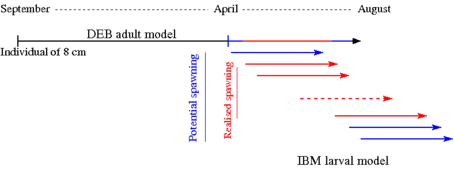
Figure 1: Schematic representation of the experiment with the two successive models. In blue the potential spawning, in red the realised spawning as determined by the adult DEB model.
