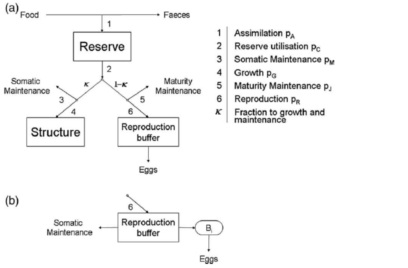
Figure 3: (a) Energy fluxes through an individual at the adult stage following DEB theory and (b) specific handling rules of the reproduction buffer (Pecquerie et al. 2009): somatic maintenance can be paid from the reproduction buffer if \kappa p_C - p_M < 0 and energy is allocated from the reproduction buffer to the successive batches of eggs located in the gonads during the spawning season (the i^{th} batch is represented).
