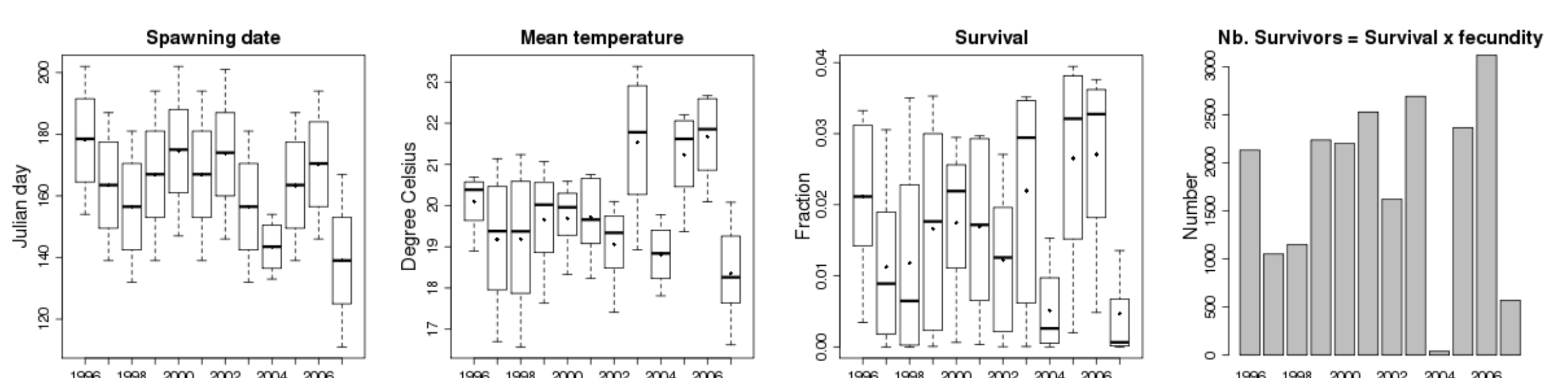
Figure 10: Same as Fig. 7 for spawning in zone 2.
